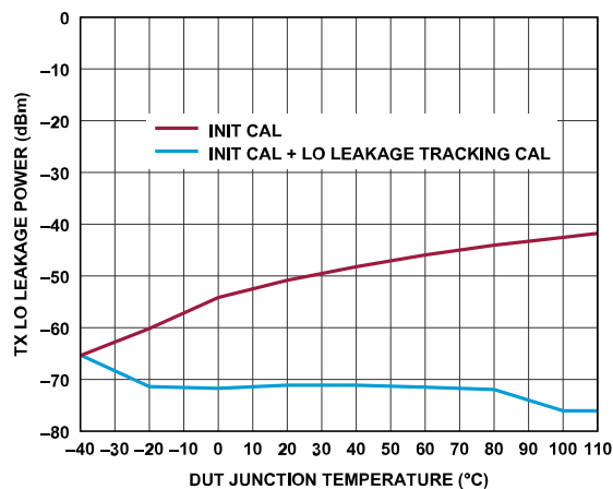
Figure 104. Transmitter LO Leakage Power vs. DUT Junction Temperature (Low to High), Baseband Frequency = 4 MHz, Backoff = 0.5 dBFS, Attenuation Code = 0
