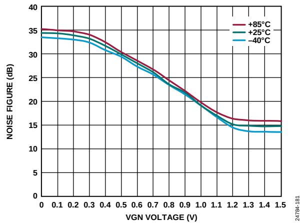
Figure 73. Noise Figure vs. VGN Voltage over Temperature at 2 GHz
