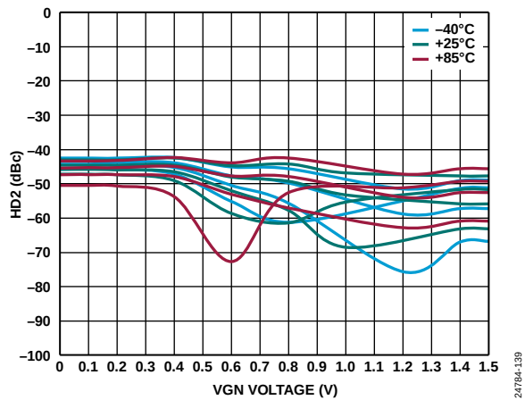
Figure 35. HD2 vs. VGN Voltage over Temperature and OFSx at 2 GHz
