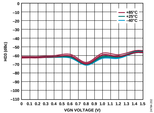
Figure 94. HD3 vs. VGN Voltage over Temperature and OFSx at 1 GHz
