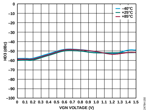
Figure 49. HD3 vs. VGN Voltage over Temperature and VOCM at 3 GHz
