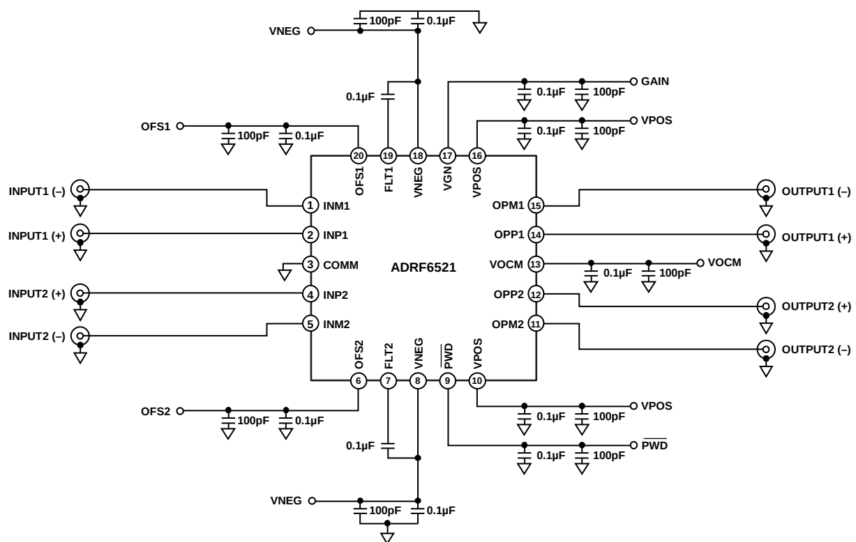
Figure 125. Basic Connections
