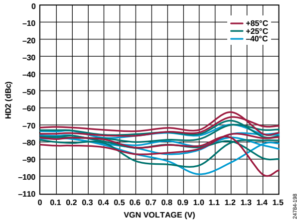
Figure 90. HD2 vs. VGN Voltage over Temperature and OFSx at 500 MHz
