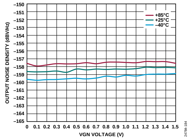
Figure 76. Output Noise Density vs. VGN Voltage over Temperature at 2 GHz
