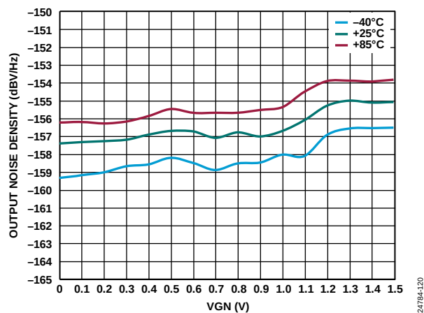
Figure 19. Output Noise Density vs. VGN over Temperature at 2 GHz
