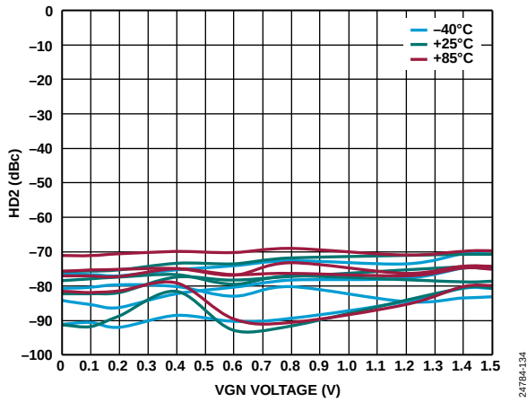
Figure 33. HD2 vs. VGN Voltage over Temperature and OFSx at 500 MHz
