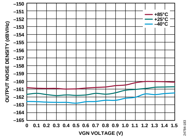
Figure 75. Output Noise Density vs. VGN Voltage over Temperature at 1 GHz
