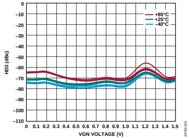
Figure 93. HD3 vs. VGN Voltage over Temperature and OFSx at 500 MHz
