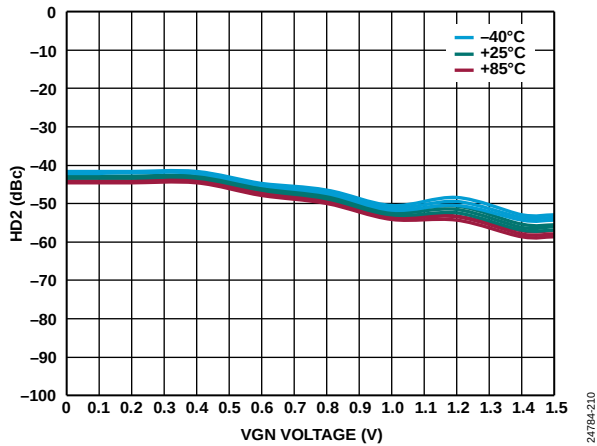
Figure 102. HD2 vs. VGN Voltage over Temperature and VOCM at 2 GHz
