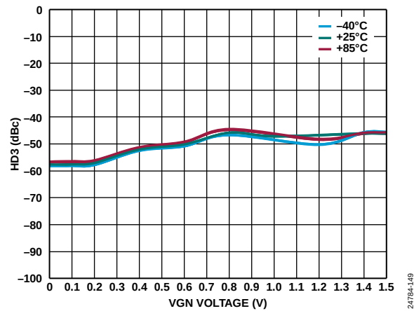
Figure 48. HD3 vs. VGN Voltage over Temperature and VOCM at 2 GHz
