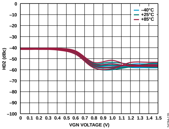
Figure 34. HD2 vs. VGN Voltage over Temperature and OFSx at 1 GHz
