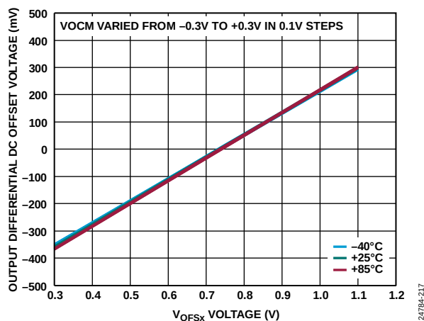
Figure 108. Output Differential DC Offset Voltage vs. V_{OFSx} Voltage over Temperature and V_OCM
