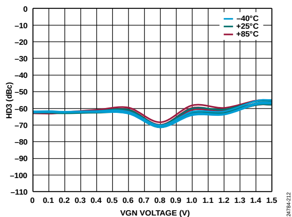
Figure 101. HD3 vs. VGN Voltage over Temperature and VOCM at 1 GHz
