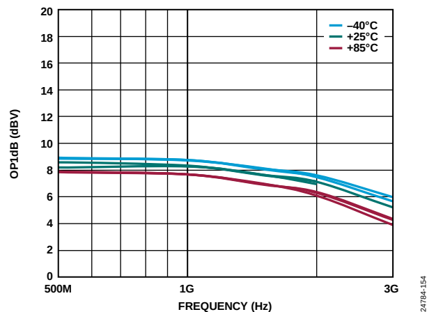
Figure 50. OP1dB vs. Frequency over Temperature and VOCM
