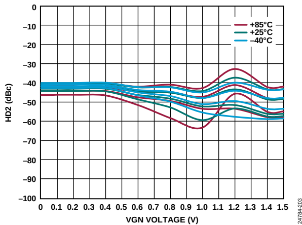
Figure 92. HD2 vs. VGN Voltage over Temperature and OFSx at 2 GHz
