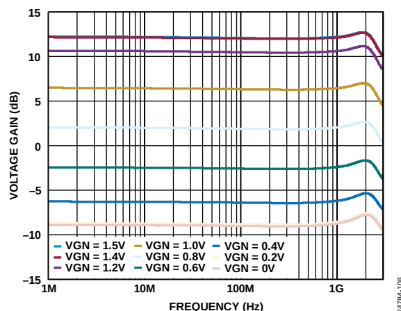
Figure 8. Voltage Gain vs. Frequency over 200 mV VGN Steps, 43 \Omega Back Terminations not De-Embedded
