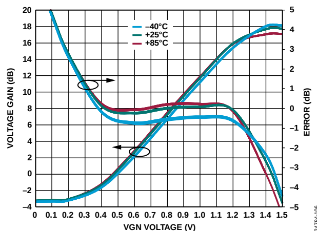
Figure 6. Voltage Gain and Error vs. VGN Voltage over Temperature at 1 GHz
