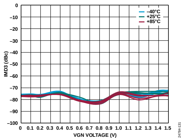
Figure 30. IMD3 vs. VGN Voltage over Temperature and OFSx at 1 GHz
