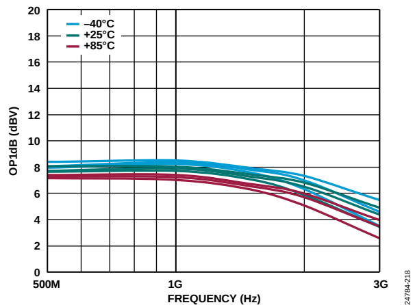
Figure 107. OP1dB vs. Frequency over Temperature and VOCM at Maximum Gain
