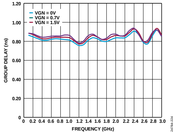
Figure 112. Group Delay vs. Frequency over VGN
