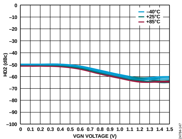
Figure 46. HD2 vs. VGN Voltage over Temperature and VOCM at 3 GHz
