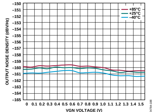
Figure 77. Output Noise Density vs. VGN Voltage over Temperature at 3 GHz
