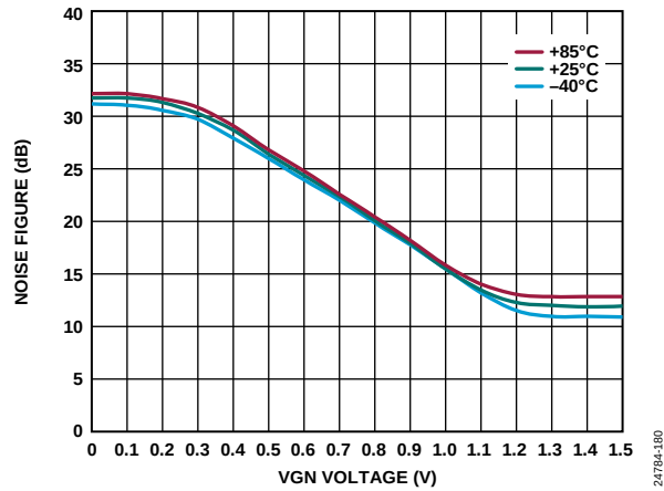
Figure 72. Noise Figure vs. VGN Voltage over Temperature at 1 GHz
