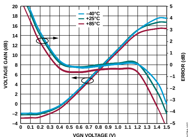
Figure 7. Voltage Gain and Error vs. VGN Voltage over Temperature at 3 GHz
