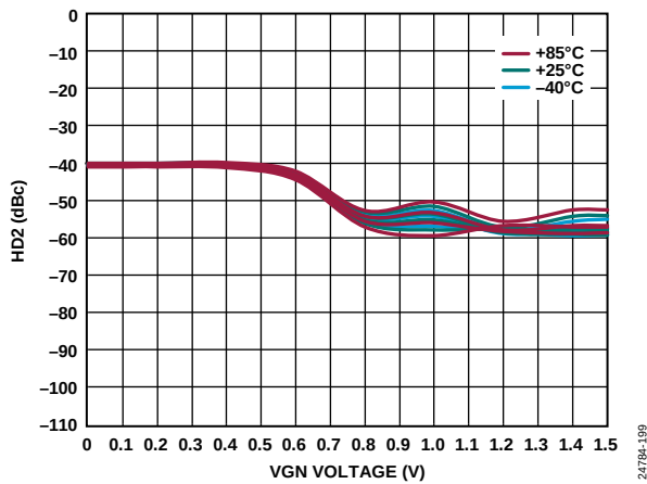
Figure 91. HD2 vs. VGN Voltage over Temperature and OFSx at 1 GHz
