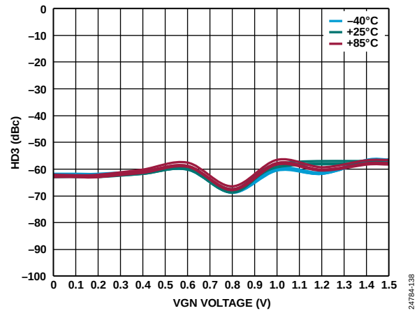
Figure 37. HD3 vs. VGN Voltage over Temperature and VDCM at 1 GHz
