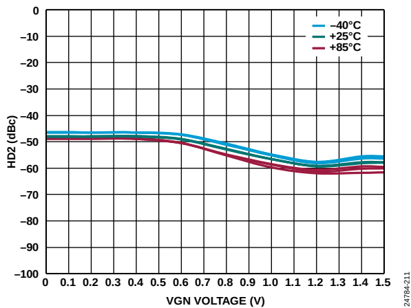
Figure 103. HD2 vs. VGN Voltage over Temperature and VOCM at 3 GHz
