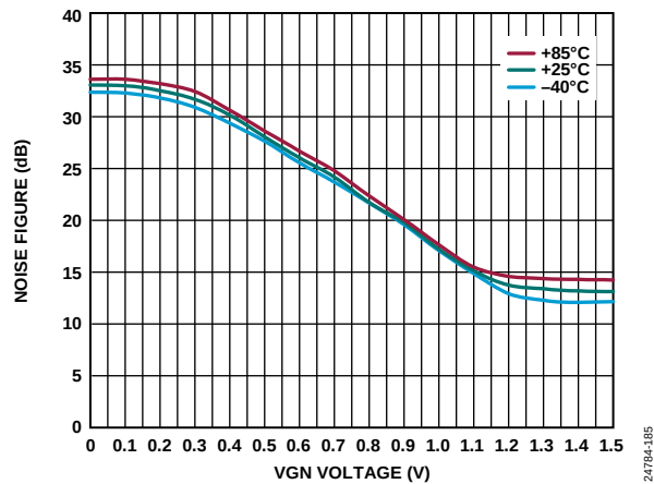
Figure 74. Noise Figure vs. VGN Voltage over Temperature at 3 GHz
