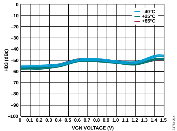
Figure 106. HD3 vs. VGN Voltage over Temperature and VOCM at 3 GHz
