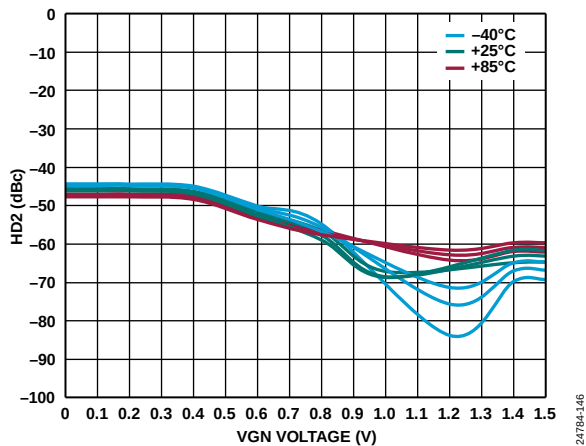
Figure 45. HD2 vs. VGN Voltage over Temperature and VOCM at 2 GHz
