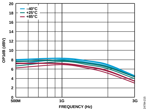
Figure 104. OP1dB vs. Frequency over Temperature and OFSx at Maximum Gain
