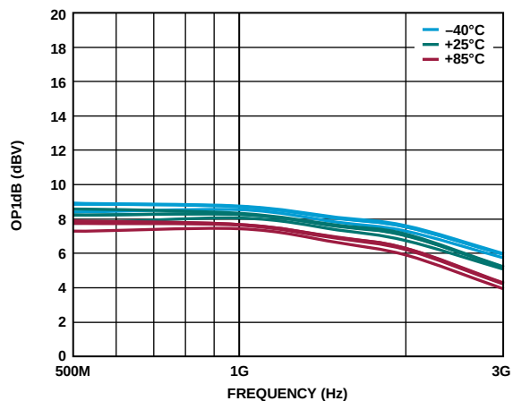
Figure 47. OP1dB vs. Frequency over Temperature and OFSx
