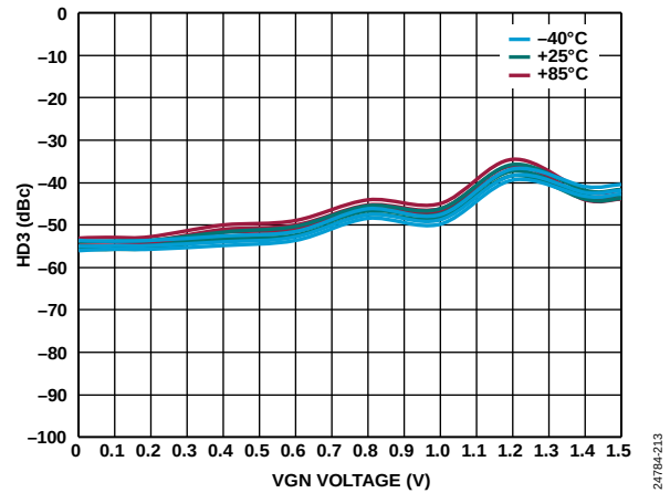
Figure 105. HD3 vs. VGN Voltage over Temperature and VOCM at 2 GHz
