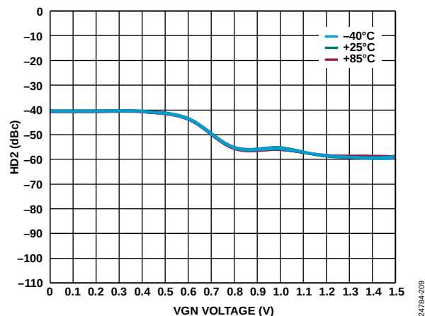
Figure 98. HD2 vs. VGN Voltage over Temperature and VOCM at 1 GHz
