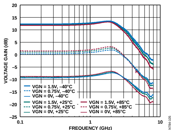
Figure 5. Voltage Gain vs. Frequency over Temperature and VGN, 43 \Omega Back Terminations not De-Embedded
