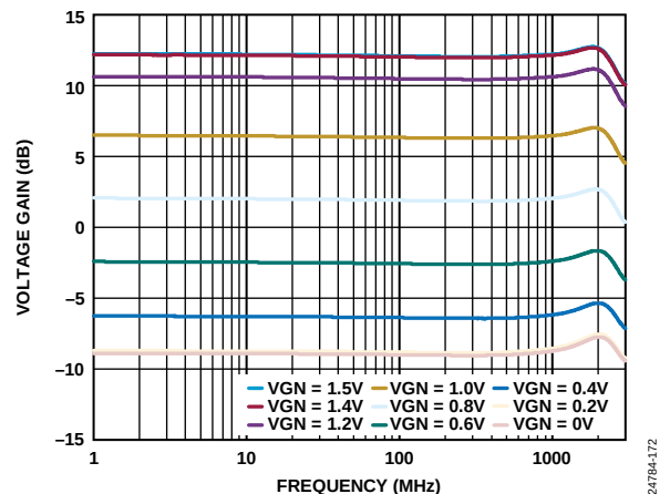
Figure 65. Voltage Gain vs. Frequency over 200 mV VGN Steps, 43 \Omega Back Terminations not De-Embedded
