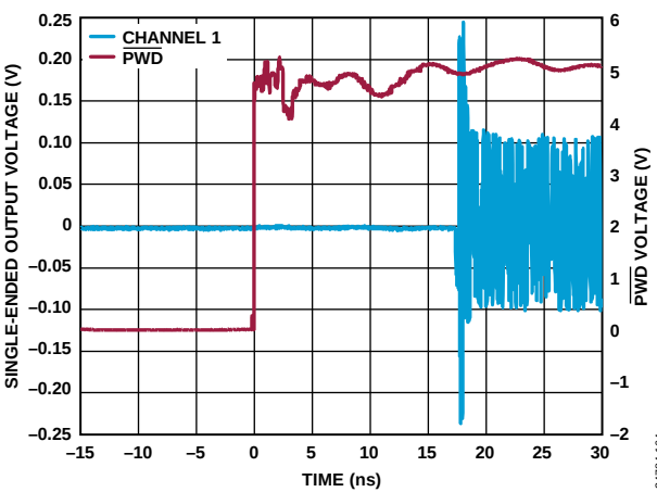
Figure 59. Enable Response Time
