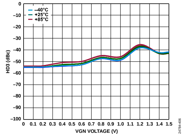
Figure 95. HD3 vs. VGN Voltage over Temperature and OFSx at 2 GHz
