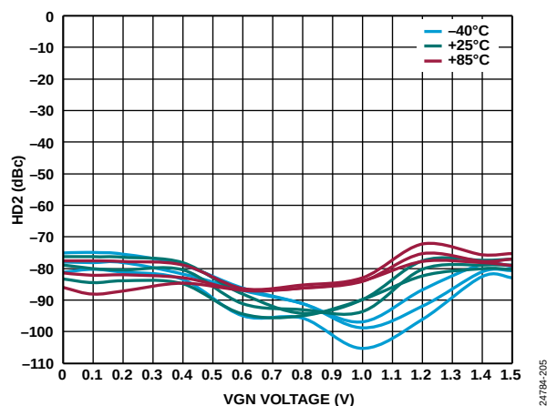
Figure 97. HD2 vs. VGN Voltage over Temperature and VOCM at 500 MHz
