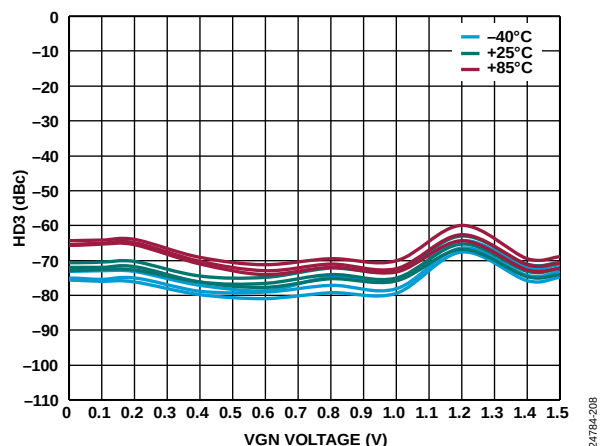
Figure 100. HD3 vs. VGN Voltage over Temperature and VOCM at 500 MHz
