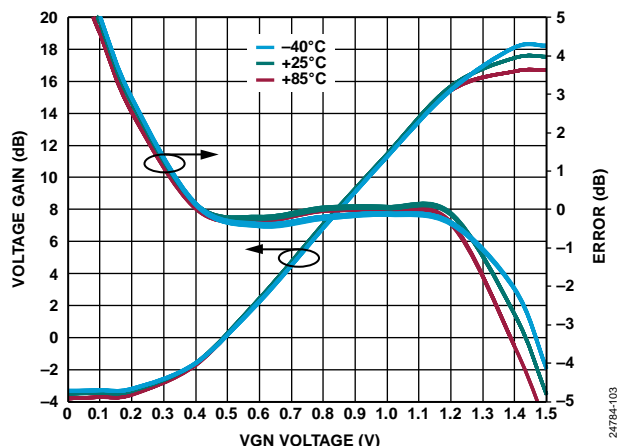
Figure 3. Voltage Gain and Error vs. VGN Voltage over Temperature at 500 MHz
