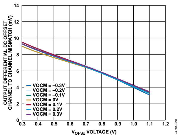
Figure 111. Output Differential DC Offset Channel to Channel Mismatch vs. V_{OFSx} Voltage over V_{OCM}
