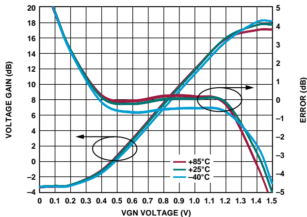
Figure 61. Voltage Gain and Error vs. VGN Voltage over Temperature at 2 GHz
