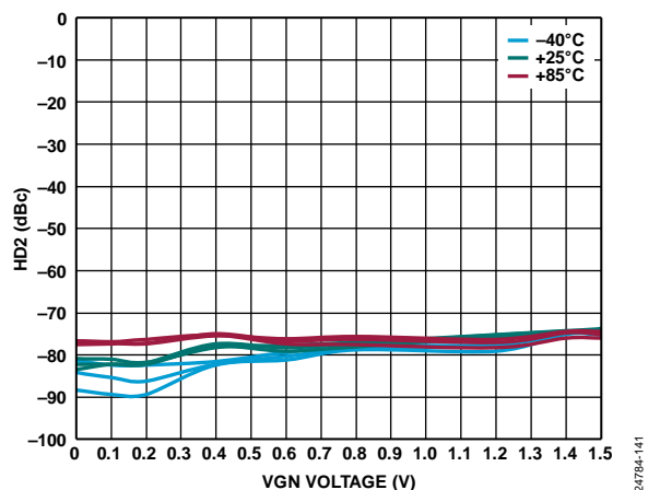
Figure 40. HD2 vs. VGN Voltage over Temperature and VOCM at 500 MHz
