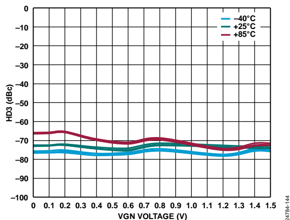
Figure 43. HD3 vs. VGN Voltage over Temperature and VOCM at 500 MHz
