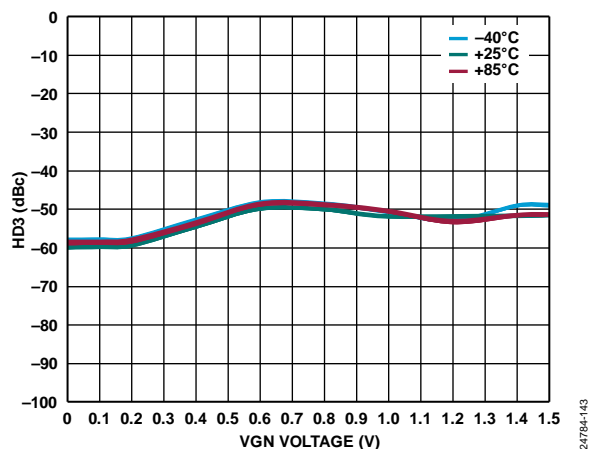
Figure 42. HD3 vs. VGN Voltage over Temperature and OFSx at 3 GHz
