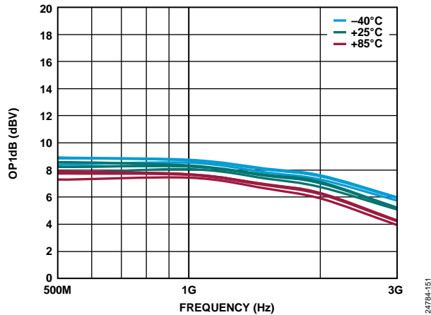
Figure 47. OP1dB vs. Frequency over Temperature and OFSx
