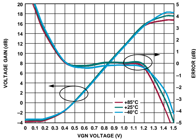
Figure 60. Voltage Gain and Error vs. VGN Voltage over Temperature at 500 MHz
