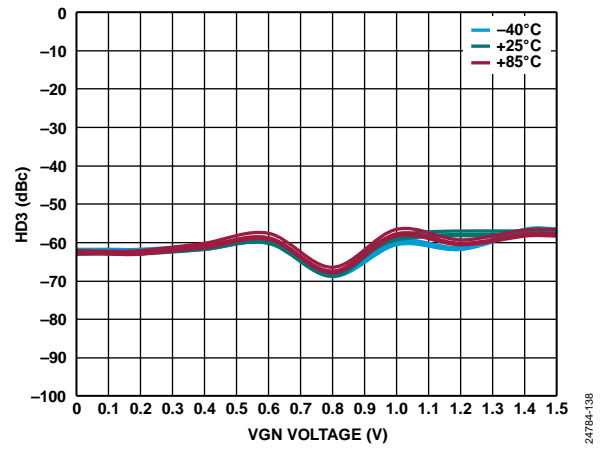
Figure 37. HD3 vs. VGN Voltage over Temperature and VOCM at 1 GHz
