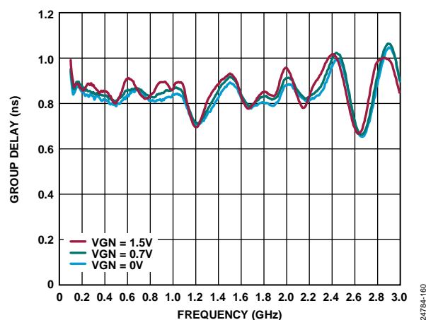
Figure 55. Group Delay vs. Frequency over VGN
