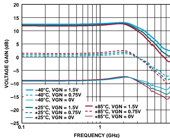
Figure 62. Voltage Gain vs. Frequency, over Temperature and VGN, 43 \Omega Back Terminations not De-Embedded
