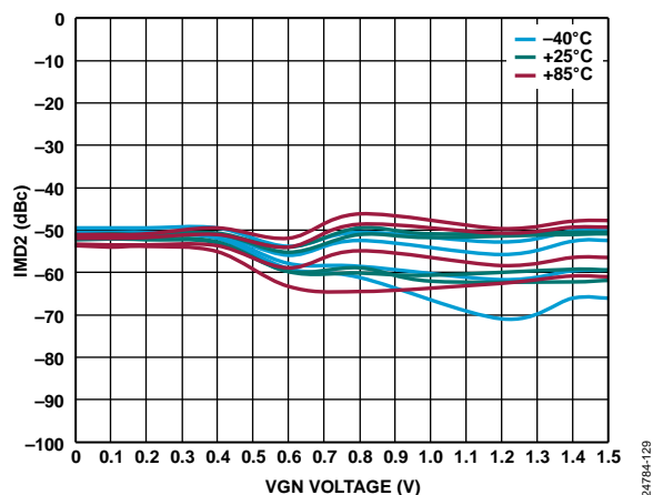
Figure 28. IMD2 vs. VGN Voltage, over Temperature and OFSx at 2 GHz
