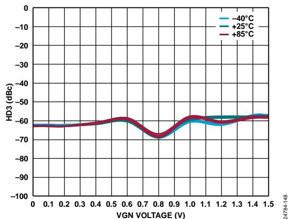
Figure 44. HD3 vs. VGN Voltage over Temperature and VOCM at 1 GHz
