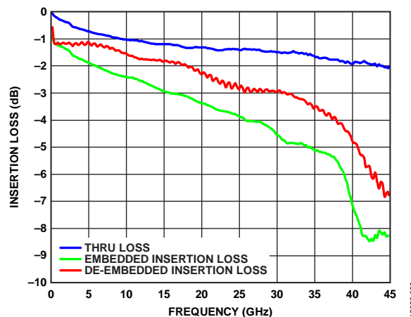
Figure 37. Insertion Loss vs. Frequency
