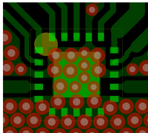
Figure 27. PCB Routings
