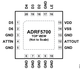
Figure 4. Pin Configuration
