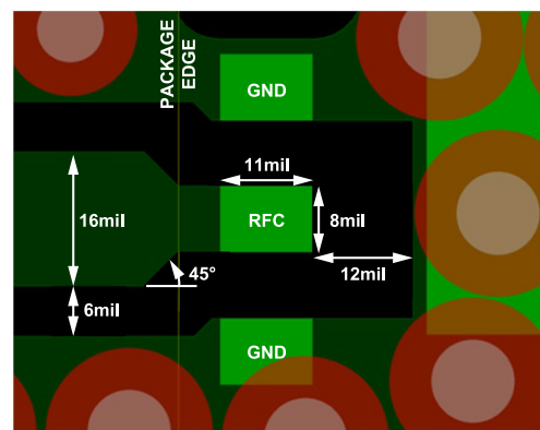
Figure 28. Recommended RF Pin Transitions
