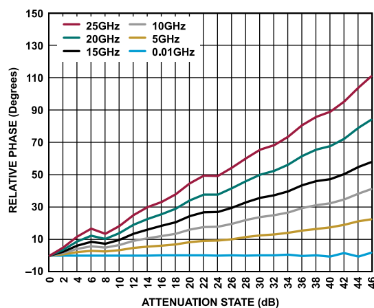
Figure 18. Relative Phase vs. Attenuation State over Frequency
