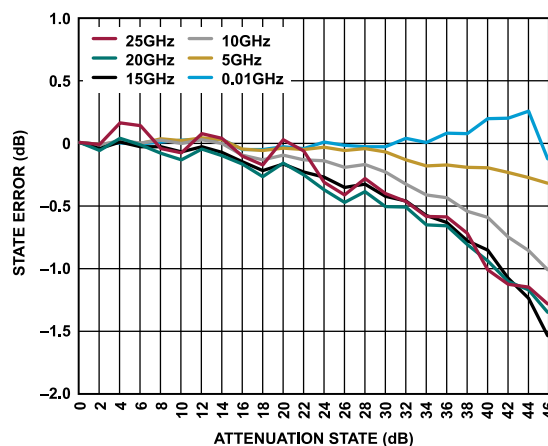
Figure 17. State Error vs. Attenuation State over Frequency
