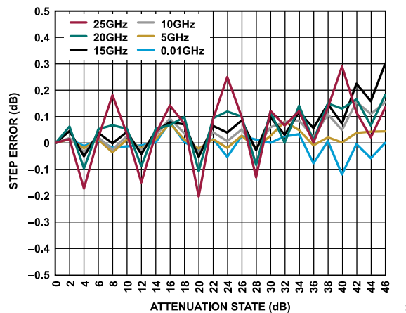
Figure 14. Step Error vs. Attenuation State over Frequency
