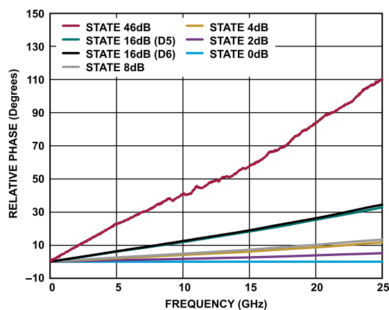
Figure 16. Relative Phase vs. Frequency
