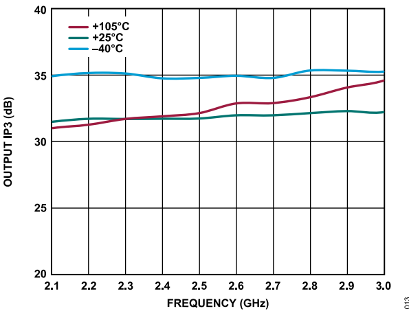
Figure 15. Output IP3 vs. Frequency, 8 dBm Output Tone Power
