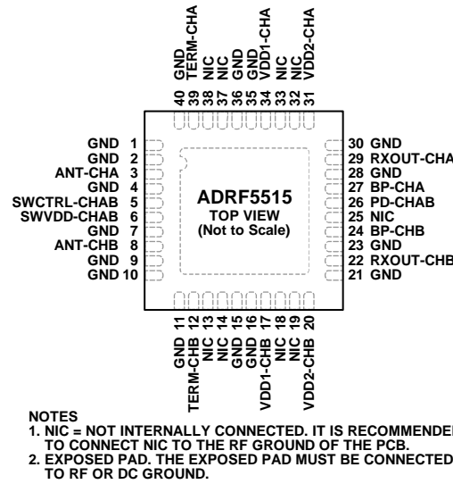
Figure 2. Pin Configuration
