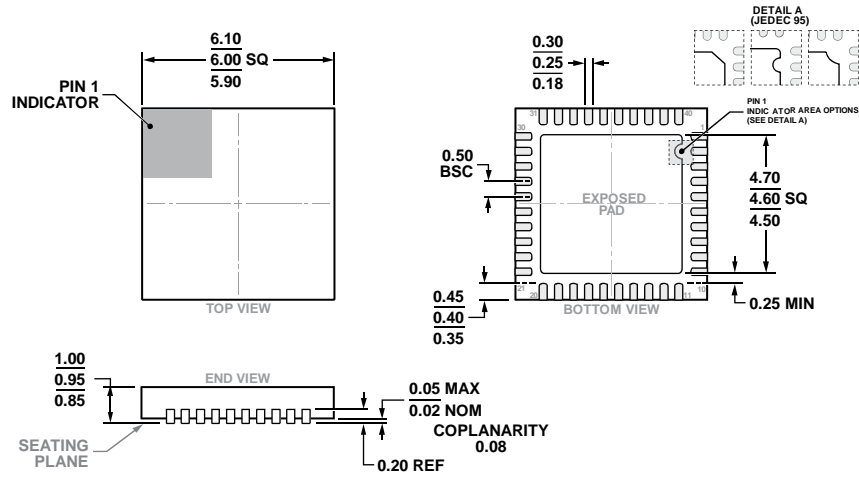
Figure 28. 40-Lead Lead Frame Chip Scale Package [LFCSP] 6 mm × 6 mm Body and 0.95 mm Package Height (CP-40-15)
