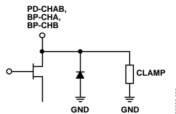
Figure 6. PD-CHAB, BP-CHA, BP-CHB Interface
