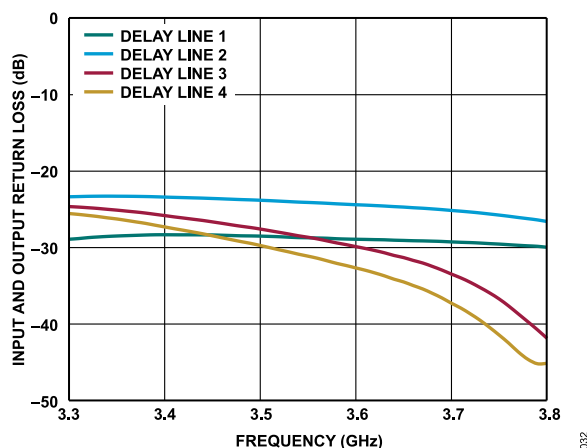
Figure 32. Input and Output Return Loss vs. Frequency
