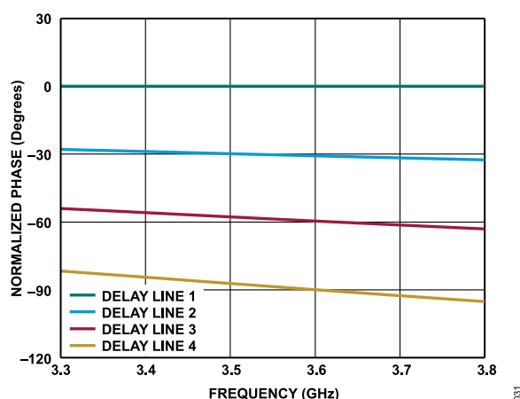
Figure 31. Back-to-Back Normalized Phase vs. Frequency
