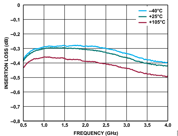
Figure 8. Insertion Loss for RFC to RF1 vs. Frequency over Temperature
