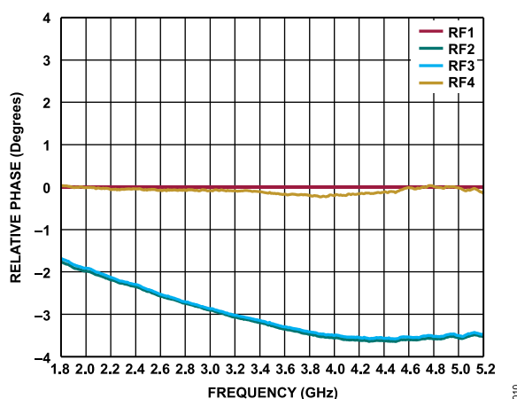
Figure 10. Relative Phase RFC - RFx Normalized to RFC - RF1
