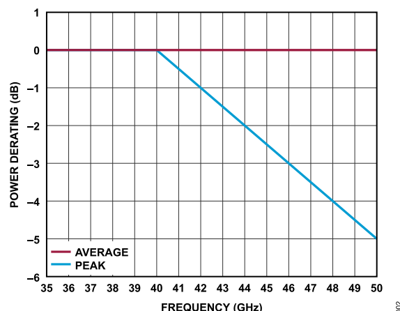
Figure 2. Power Derating vs. Frequency, T CASE = +85°C
