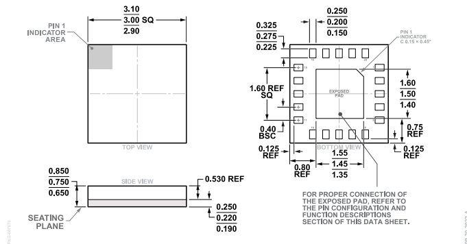
Figure 18. 20-Terminal Land Grid Array [LGA] 3 mm x 3 mm Body and 0.75 mm Package Height (CC-20-17) Dimensions Shown in Millimeters
