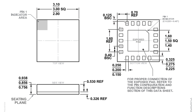
Figure 19. 20-Terminal Land Grid Array [LGA] 3.0 mm × 3.0 mm Body and 0.856 mm Package Height (CC-20-13) Dimensions Shown in millimeters
