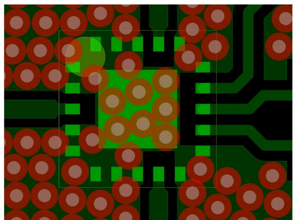
Figure 17. PCB Routings
