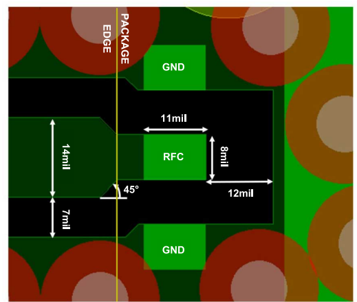
Figure 18. Recommended RF Pin Transitions
