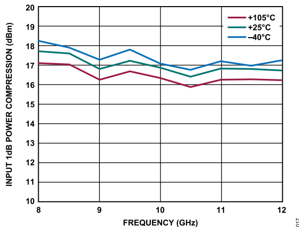
Figure 16. Input 1dB Power Compression vs. Frequency over Temperature for RX
