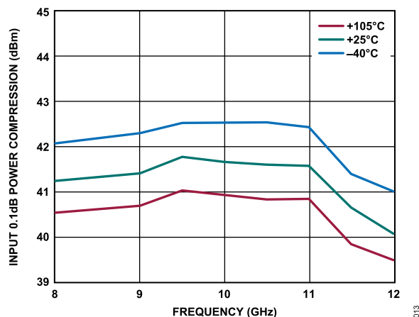
Figure 13. Input 0.1dB Power Compression vs. Frequency over Temperature for TX
