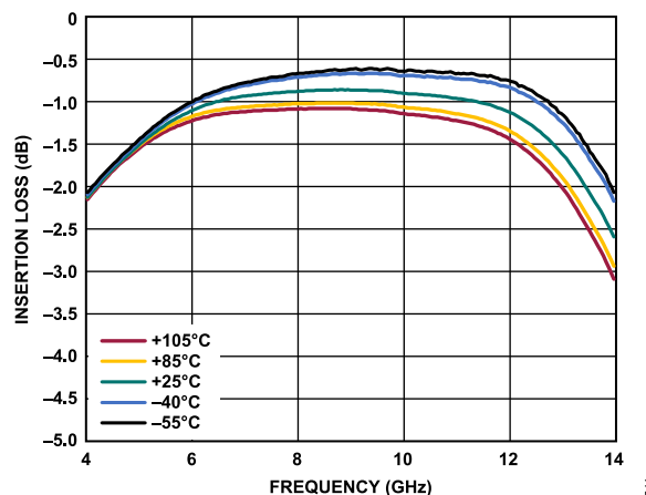
Figure 11. Insertion Loss vs. Frequency over Temperature for TX
