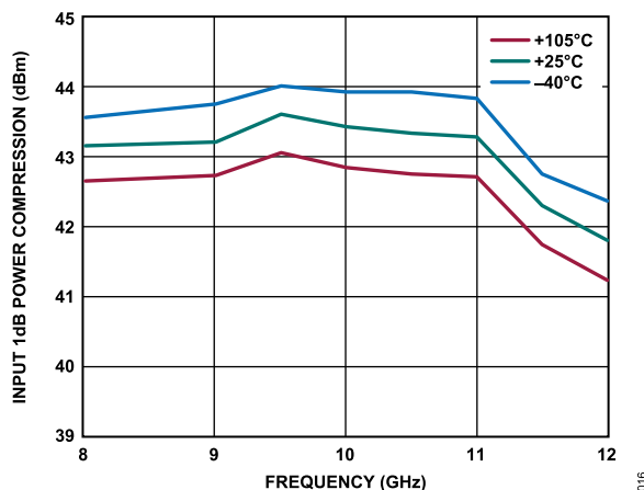
Figure 15. Input 1dB Power Compression vs. Frequency over Temperature for TX
