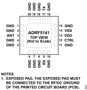
Figure 3. Pin Configuration (Top View)
