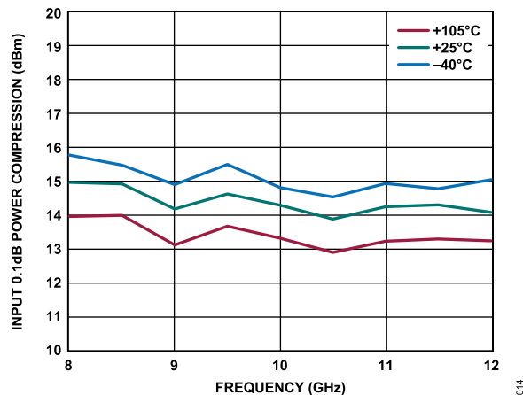
Figure 14. Input 0.1dB Power Compression vs. Frequency over Temperature for RX
