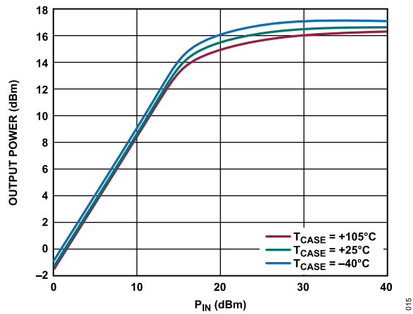
Figure 17. Output Power ( P_{OUT} ) vs. P_{IN} over Temperature at 10 GHz for RX
