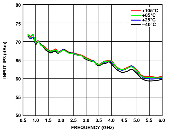
Figure 10. Input IP3 vs. Frequency over Temperature, V_{DD} = 5\text{ V}
