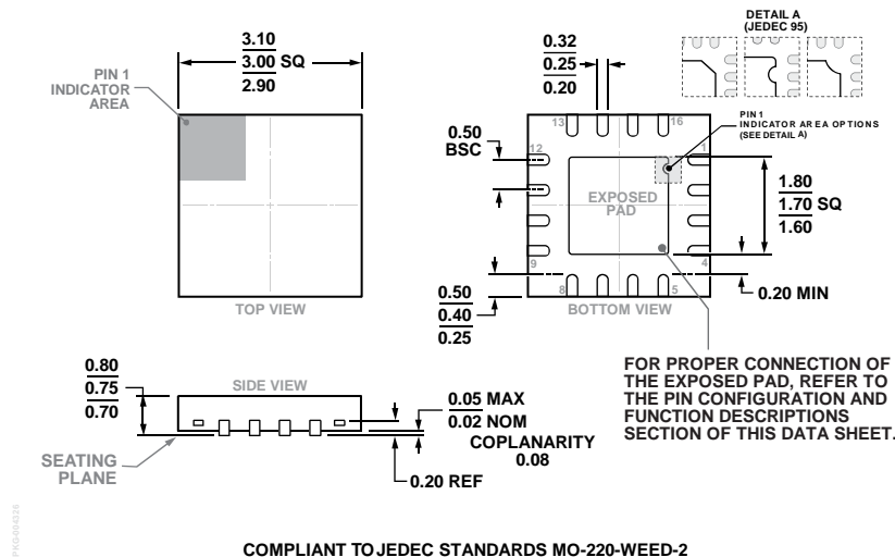
Figure 18. 16-Lead Lead Frame Chip Scale Package [LFCSP] 3 mm × 3 mm Body and 0.75 mm Package Height (CP-16-35) Dimensions shown in millimeters
