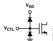
Figure 4. Control Interface
