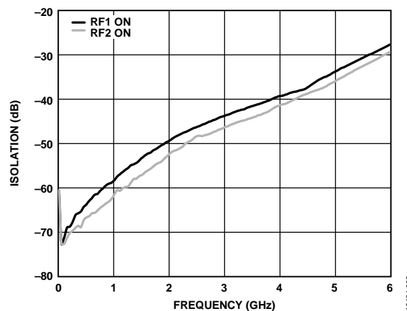
Figure 9. Isolation Between RF1 and RF2 vs. Frequency at V_{DD} = 5\text{ V} , Switch Mode On
