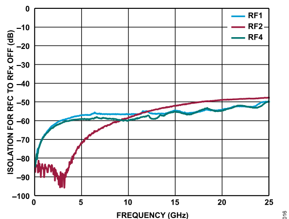
Figure 16. Isolation for RFC to RFx Off vs. Frequency, RFC to RF3 Path On
