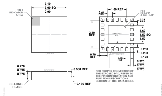
Figure 30. 24-Terminal Land Grid Array [LGA] (CC-24-16) Dimensions shown in millimeters
