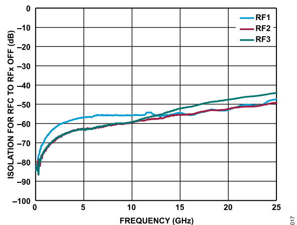
Figure 17. Isolation for RFC to RFx Off vs. Frequency, RFC to R4 Path On
