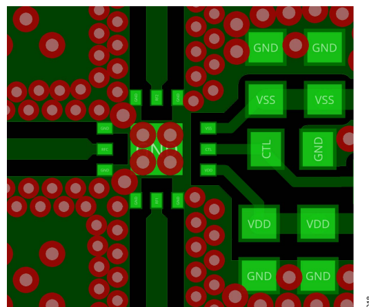
Figure 18. PCB Layout
