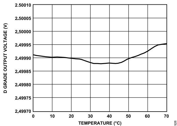
Figure 20. ADR4525 D Grade Output Voltage vs. Temperature
