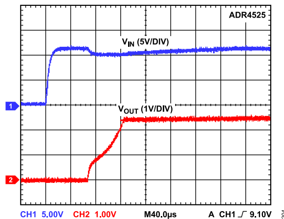
Figure 21. ADR4525 Output Voltage Start-Up Response
