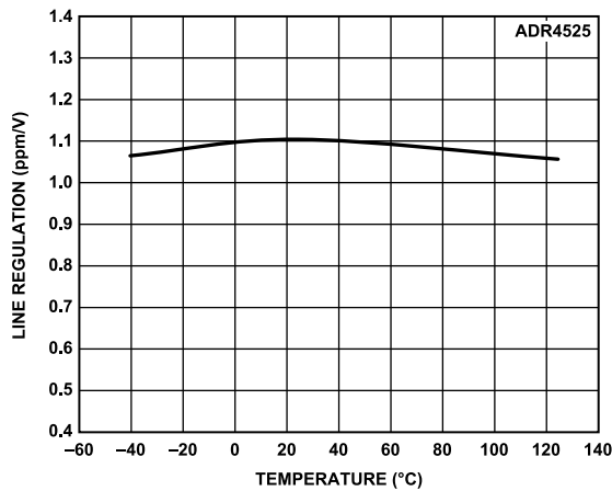
Figure 25. ADR4525 Line Regulation vs. Temperature
