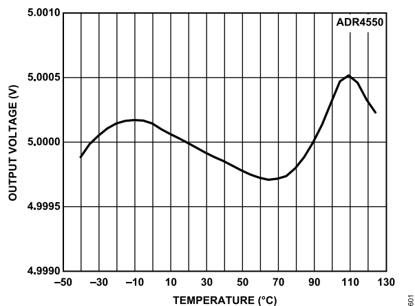
Figure 86. ADR4550 B Grade Output Voltage vs. Temperature
