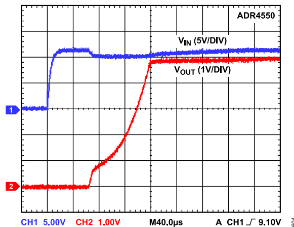
Figure 89. ADR4550 Output Voltage Start-Up Response
