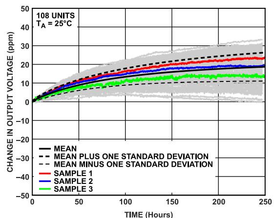
Figure 111. Measured Early Life Drift of the ADR4520/ADR4525/ADR4530/ADR4533/ADR4540/ADR4550
