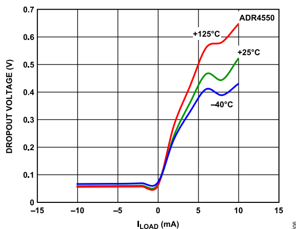
Figure 90. ADR4550 Dropout Voltage vs. Load Current
