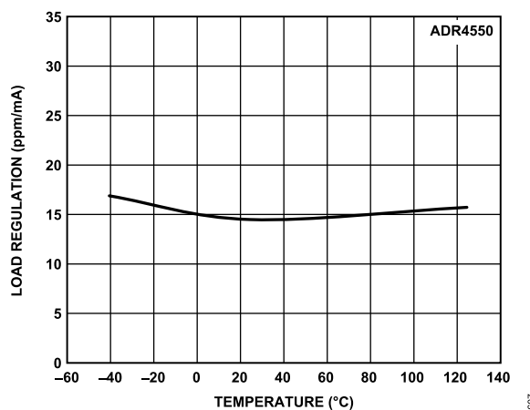
Figure 91. ADR4550 Load Regulation vs. Temperature (Sourcing)
