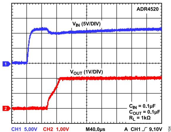
Figure 6. ADR4520 Output Voltage Start-Up Response
