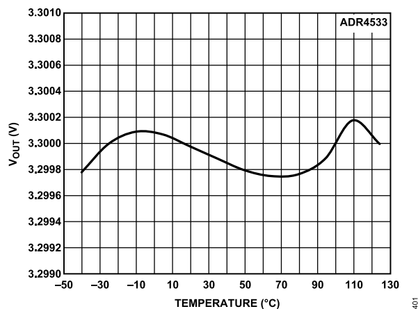
Figure 52. ADR4533 B Grade Output Voltage vs. Temperature
