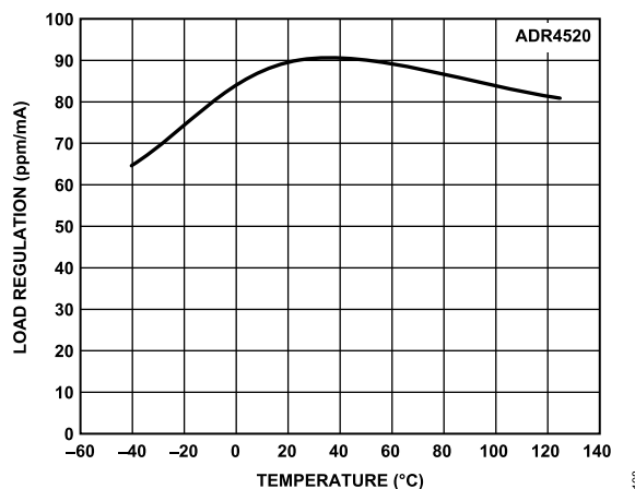
Figure 9. ADR4520 Load Regulation vs. Temperature (Sinking)
