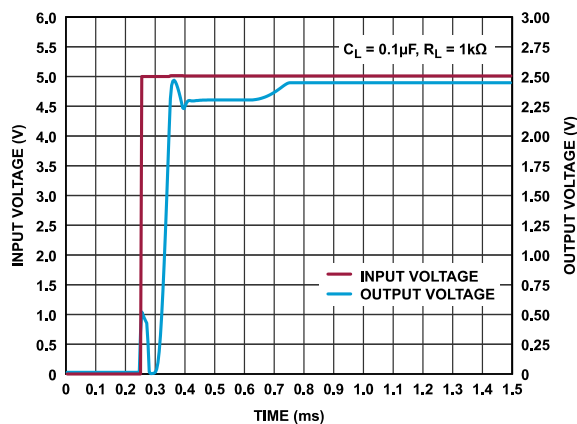
Figure 31. ADR3625 Start-Up Response (Input)
