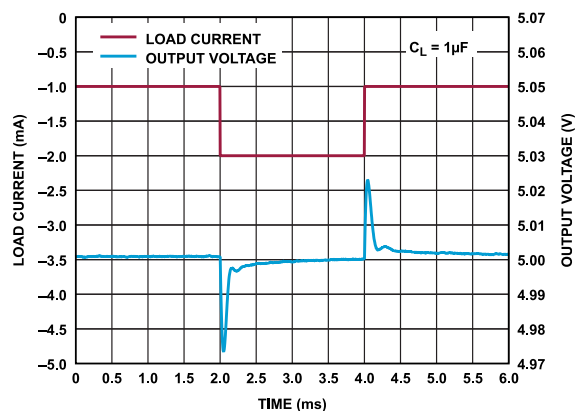
Figure 30. ADR3650 Load Transient Response (Source)
