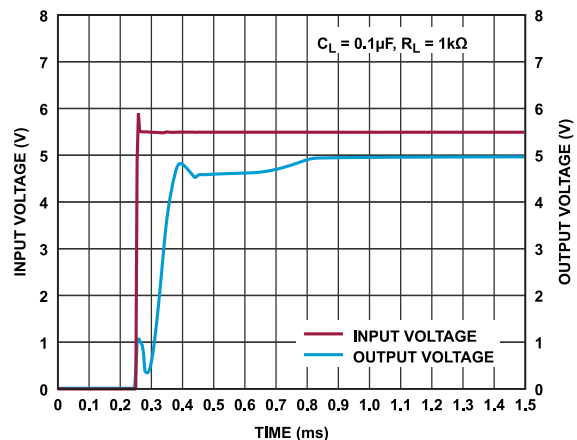
Figure 32. ADR3650 Start-Up Response (Input)
