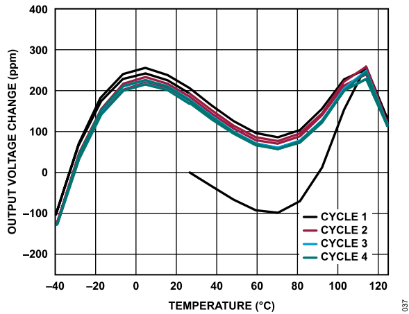
Figure 58. ADR3625 Hysteresis
