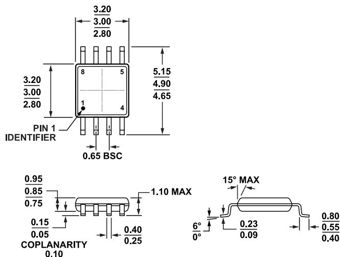
Figure 81. 8-Lead Mini Small Outline Package [MSOP] (RM-8)
