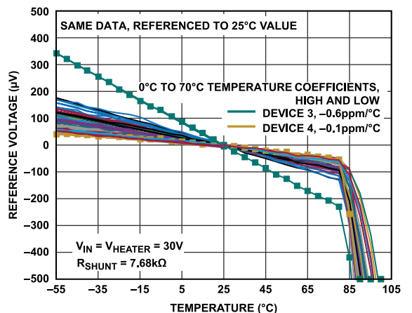
Figure 22. Reference Voltage vs. Temperature for 39 Devices, TO-46, Referenced to 25°C Value
