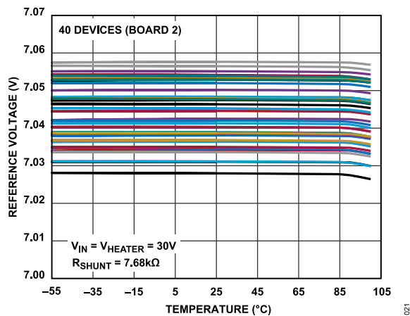
Figure 23. Reference Voltage vs. Temperature for 40 Devices, LCC
