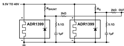
Figure 40. Parallel References for Lower Noise
