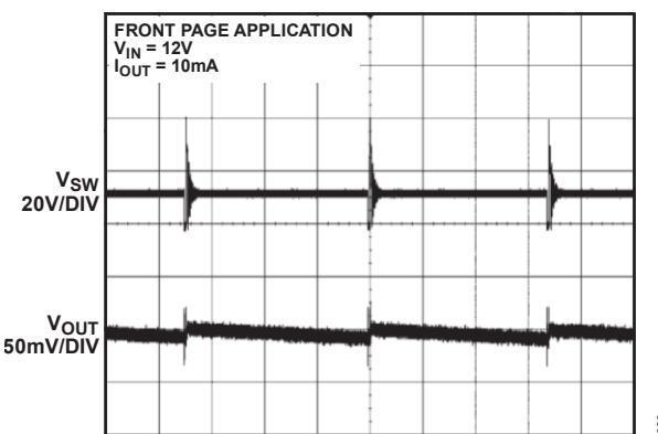
Figure 10. Burst Mode Waveforms
