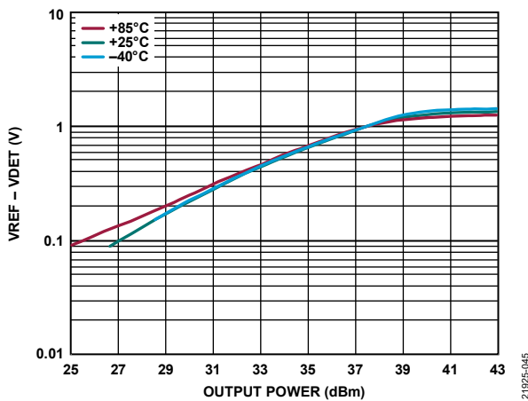
Figure 45. Detector Voltage ( V_{REF} - V_{DET} ) vs. Output Power for Various Temperatures at 1.2 GHz
