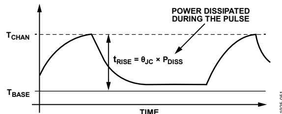
Figure 52. Pulsed Bias at Low Duty Cycle
