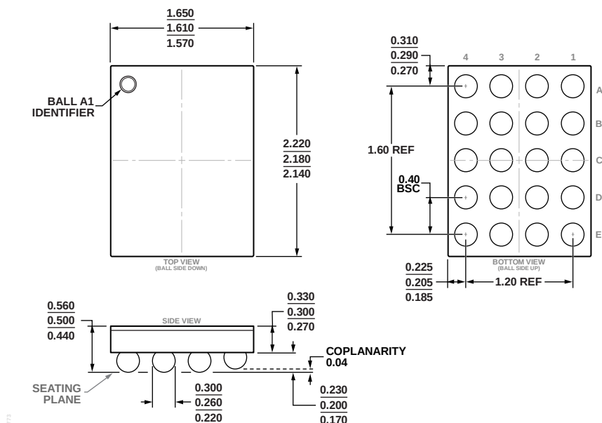
Figure 49. 20-Ball Wafer Level Chip Scale Package [WLCSP] (CB-20-14)
