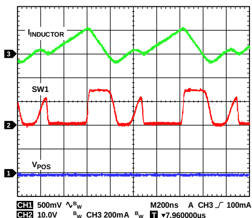
Figure 34. Boost Regulator Discontinuous Conduction Mode Operation Showing Inductor Current ( I_{INDUCTOR} ), Switch Node Voltage, and Output Ripple, V_{IN} = 5\text{ V} , V_{POS} = 15\text{ V} , I_{LOAD1} = 6\text{ mA} , f_{SW} = 2.4\text{ MHz} , T_A = 25^\circ\text{C}
