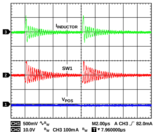
Figure 33. Boost Regulator Skip Mode Operation Showing Inductor Current ( I_{INDUCTOR} ), Switch Node Voltage, and Output Ripple, V_{IN} = 5\text{ V} , V_{POS} = 15\text{ V} , I_{LOAD1} = 4\text{ mA} , f_{SW} = 2.4\text{ MHz} , T_A = 25^\circ\text{C}
