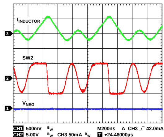
Figure 37. Inverting Regulator Discontinuous Conduction Mode Operation Showing Inductor Current ( I_{INDUCTOR} ), Switch Node Voltage, and Output Ripple, V_{IN} = 5\text{ V} , V_{NEG} = -5\text{ V} , I_{LOAD2} = 6\text{ mA} , f_{SW} = 2.4\text{ MHz} , T_A = 25^\circ\text{C}
