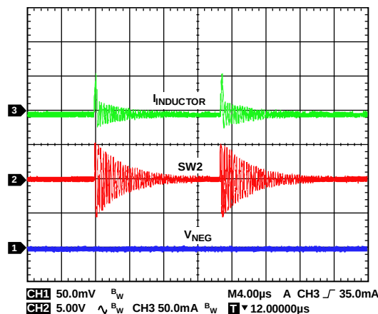
Figure 36. Inverting Regulator Skip Mode Operation Showing Inductor Current ( I_{INDUCTOR} ), Switch Node Voltage, and Output Ripple, V_{IN} = 5\text{ V} , V_{NEG} = -5\text{ V} , I_{LOAD2} = 0\text{ mA} , f_{SW} = 2.4\text{ MHz} , T_A = 25^\circ\text{C}
