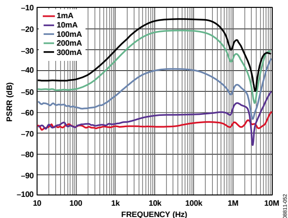
Figure 53. LDO2 PSRR Across Output Load, VIN3 = 3.6 V, VOUT3 = 3.3 V
