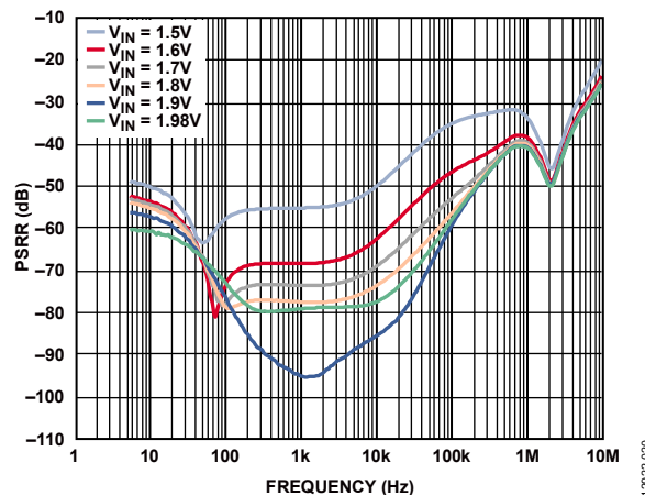
Figure 20. Power Supply Rejection Ratio (PSRR) vs. Frequency for Various V_{IN} , V_{OUT} = 1.3 V, Load Current = 2 A
