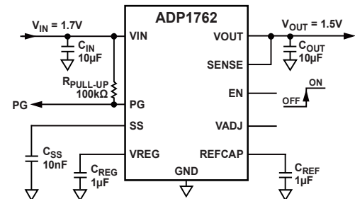
Figure 1. Fixed Output Operation
