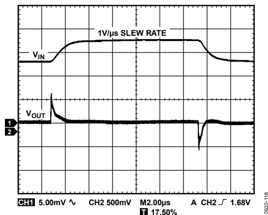
Figure 16. Line Transient Response, Load Current = 2 A, V_{IN} = 1.5 V to 1.98 V Step, V_{OUT} = 1.3 V
