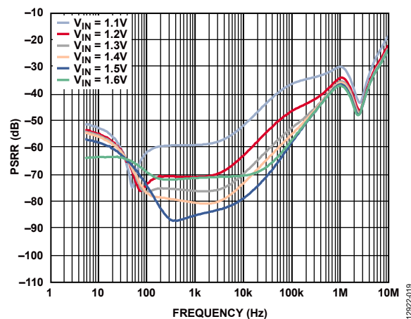
Figure 19. Power Supply Rejection Ratio (PSRR) vs. Frequency for Various V_{IN} , V_{OUT} = 0.9 V, Load Current = 2 A
