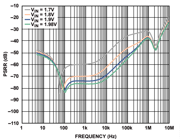
Figure 21. Power Supply Rejection Ratio (PSRR) vs. Frequency for Various V_{IN} , V_{OUT} = 1.5 V, Load Current = 2 A
