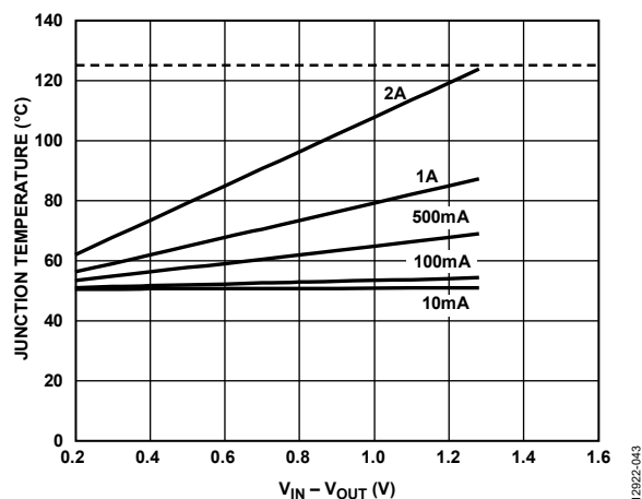
Figure 43. 1000 mm 2 of PCB Copper, T_B = 50^\circ\text{C}
