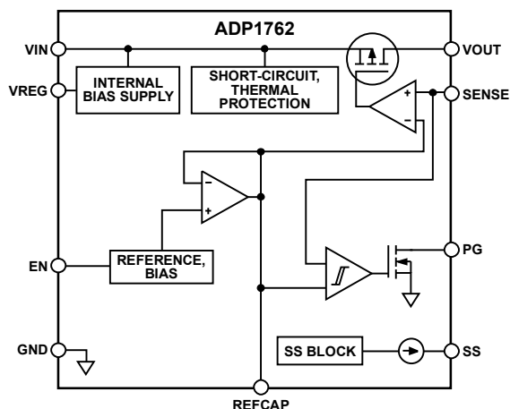
Figure 23. Functional Block Diagram, Fixed Output
