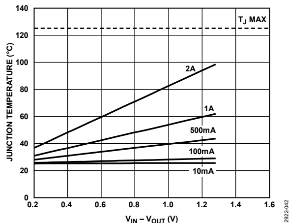
Figure 42. 1000 mm 2 of PCB Copper, T_B = 25^\circ\text{C}
