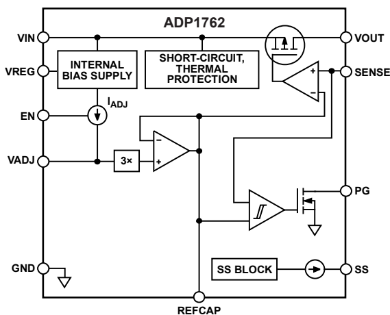
Figure 24. Functional Block Diagram, Adjustable Output
