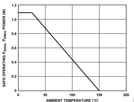
Figure 2. Thermal Derivative Curve, Dependence of Safety Limiting Values with Ambient Temperature per DIN VDE V 0884-10
