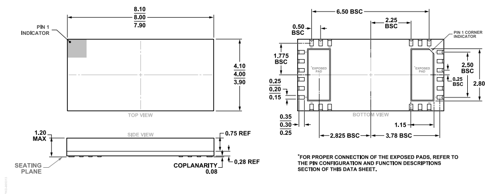
Figure 29. 24-Terminal Land Grid Array [LGA] (CC-24-6) Dimensions shown in millimeters
