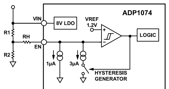
Figure 14. Precision EN with Adjustable Hysteresis
