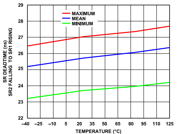
Figure 11. SR Dead Time (SR2 Falling to SR1 Rising) vs. Temperature
