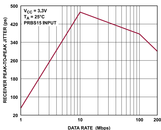
Figure 16. Receiver Peak-to-Peak Jitter vs. Data Rate ( V_{ID} = 400 mV, V_{IC} = 1.1 V)
