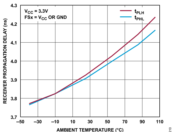
Figure 10. Receiver Propagation Delay vs. Ambient Temperature ( V_{ID} = 400 \text{ mV} and V_{IC} = 1.1 \text{ V} )
