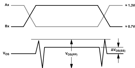
NOTES 1. INPUT PULSE GENERATOR: 1MHz; 50% \pm 5% DUTY CYCLE; t_R, t_F \leq 1 ns. 2. V_{OS(PP)} MEASURED ON TEST EQUIPMENT WITH -3 dB BANDWIDTH \geq 1 GHz.
