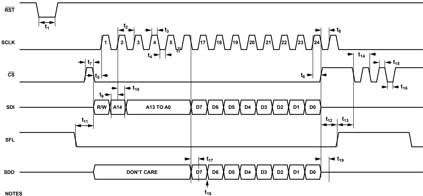
Figure 2. Timing Diagram
