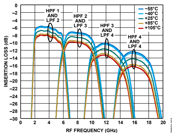
Figure 7. Insertion Loss vs. RF Frequency at 4 GHz Constant Bandwidth and Various Temperatures
