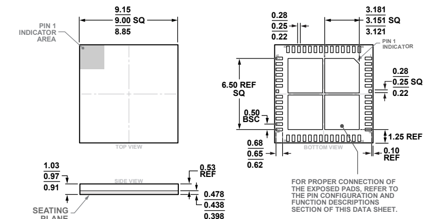
Figure 38. 56-Terminal Land Grid Array [LGA] 9 mm x 9 mm Body and 0.97 mm Package Height (CC-56-3) Dimensions shown in millimeters
