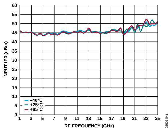
Figure 18. Input IP3 vs. RF Frequency for Various Temperatures, Bypass Configuration
