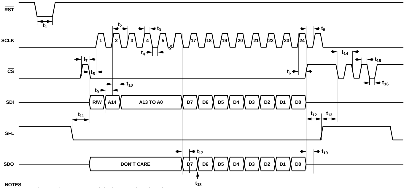
Figure 2. Timing Diagram
