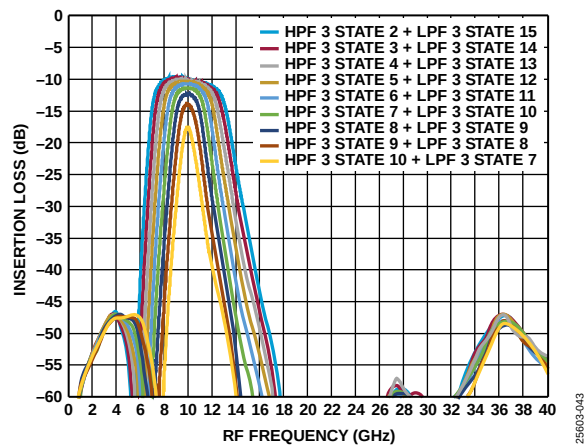
Figure 27. Insertion Loss vs. RF Frequency, Center Frequency ( f_{\text{CENTER}} ) = 10 GHz in Various 3 dB Bandwidth for HPF 3 and LPF 3 Configuration
