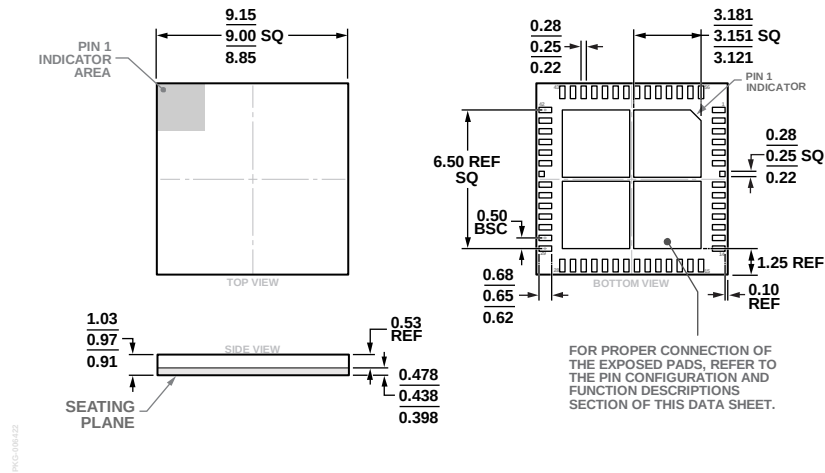
Figure 38. 56-Terminal Land Grid Array [LGA] 9 mm × 9 mm Body and 0.97 mm Package Height (CC-56-3) Dimensions shown in millimeters
