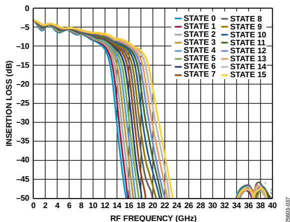
Figure 28. Insertion Loss vs. RF Frequency, LPF 3 Configuration Swept LPF State
