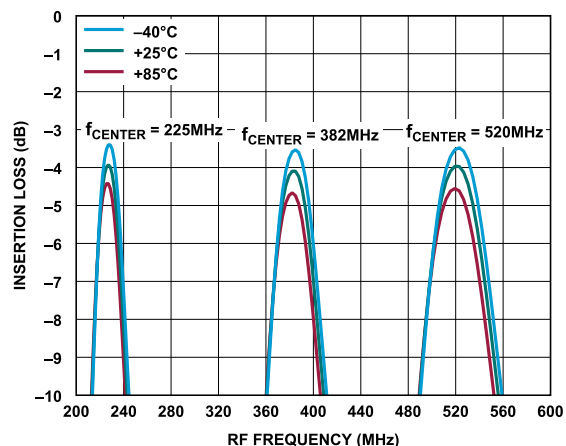
Figure 35. Insertion Loss vs. RF Frequency for Nominal Bandwidth and Various Temperatures and Center Frequencies
