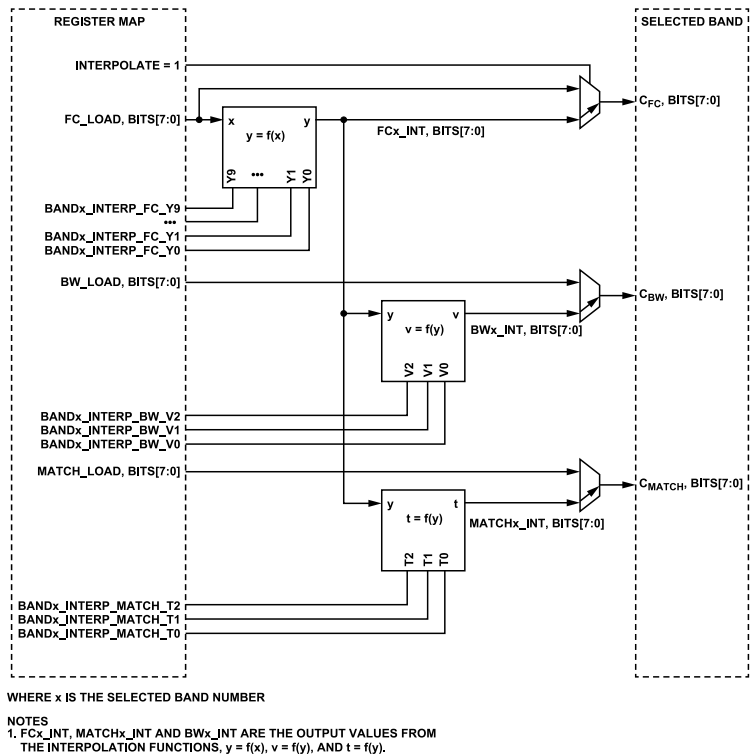
Figure 51. Interpolation Diagram
