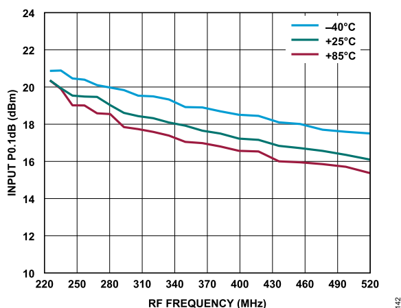
Figure 42. Input P0.1dB vs. RF Frequency for Nominal Bandwidth and Various Temperatures
