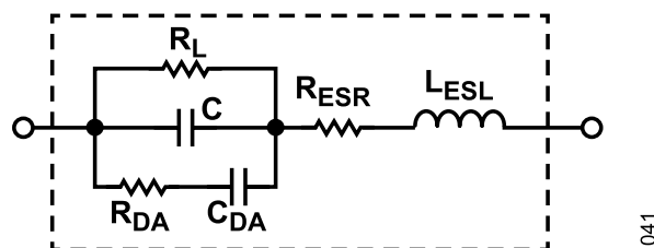
Figure 49. Model of a Capacitor
