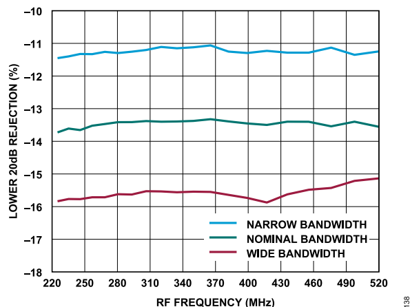
Figure 38. Percentage Away from f_{\text{CENTER}} for Lower 20 dB Rejection vs. RF Frequency for Various Bandwidths
