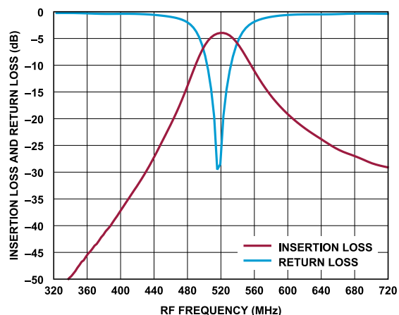
Figure 36. Insertion Loss and Return Loss vs. RF Frequency for Nominal Bandwidth at 520 MHz
