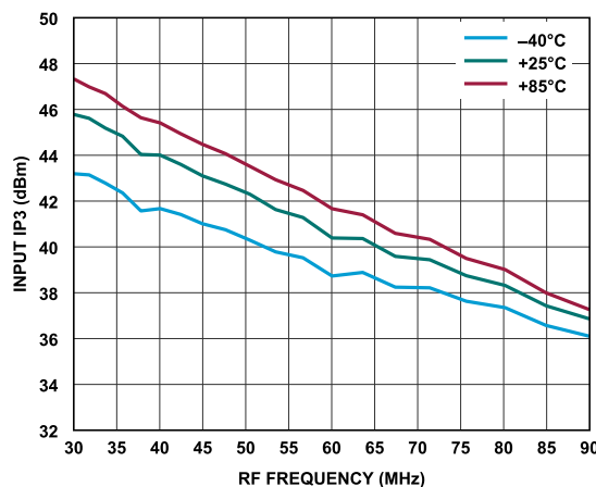
Figure 15. In-Band Input IP3 vs. RF Frequency for Nominal Bandwidth and Various Temperatures (See the Specifications Section for Further Information)
