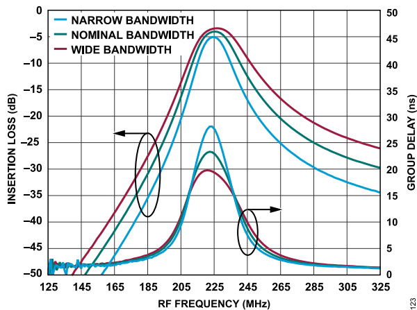
Figure 23. Insertion Loss and Group Delay vs. RF Frequency at 224.9 MHz
