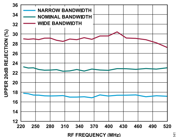
Figure 41. Percentage Away from f_{\text{CENTER}} for Upper 20 dB Rejection vs. RF Frequency for Various Bandwidths
