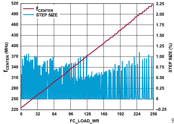
Figure 45. f_{\text{CENTER}} and Step Size vs. \text{FC\_LOAD\_WR}
