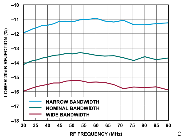
Figure 10. Percentage Away from f_{\text{CENTER}} for Lower 20 dB Rejection vs. RF Frequency for Various Bandwidths
