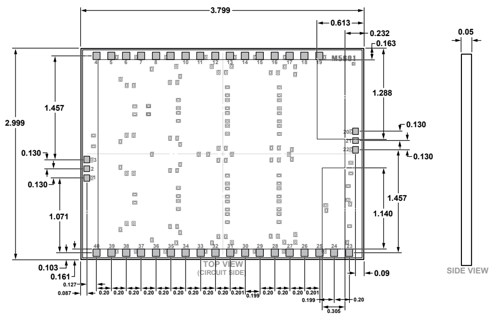
Figure 50. 40-Pad Bare Die [CHIP] (C-40-3) Dimensions shown in millimeters
