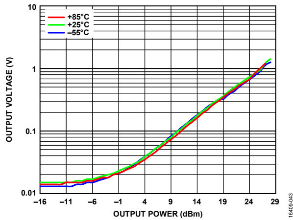
Figure 43. Detector Output Voltage ( V_{OUT} ) vs. Output Power over Various Temperatures, I_{DD} = 800 mA, RF = 83.5 GHz
