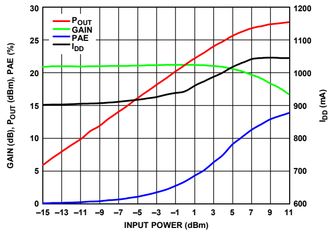
Figure 36. Gain, P_{OUT} , PAE, and I_{DD} vs. Input Power, RF = 86 GHz, I_{DD} = 900 mA
