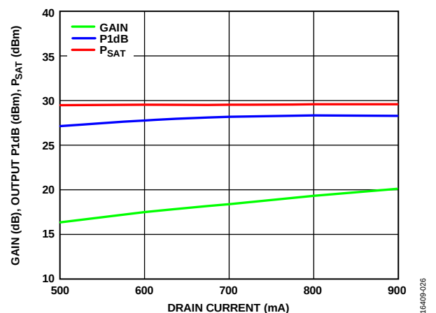
Figure 26. Gain, Output P1dB, and P_{SAT} vs. Drain Current ( I_{DD} ), RF = 83.5 GHz
