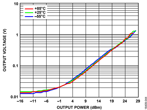
Figure 44. Detector Output Voltage ( V_{OUT} ) vs. Output Power over Temperatures, I_{DD} = 800 mA, RF = 86 GHz
