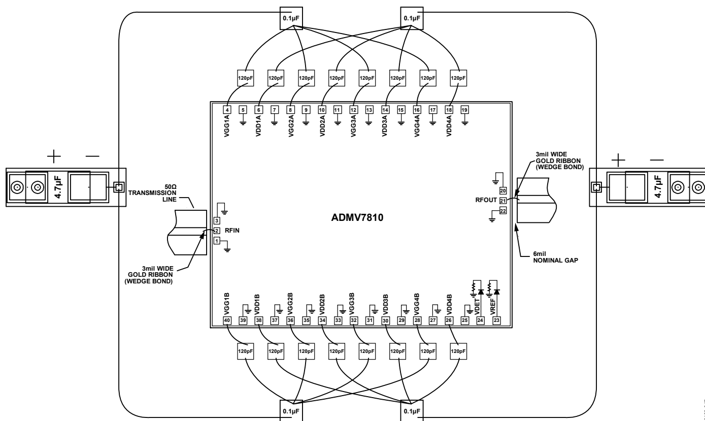
Figure 48. Assembly Diagram
