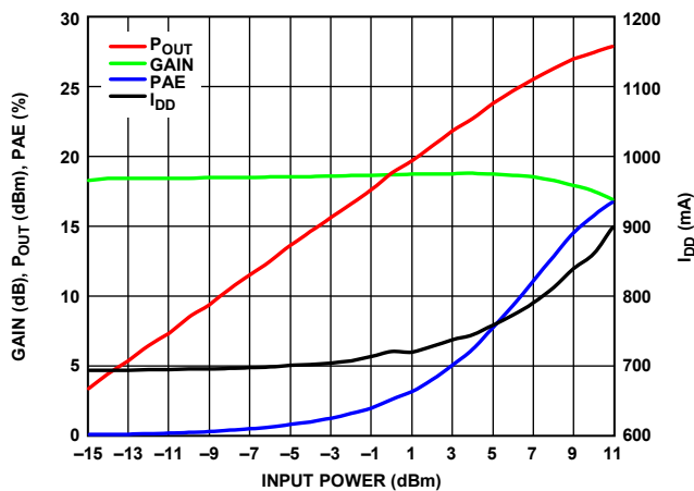
Figure 29. Gain, P_{OUT} , PAE, and I_{DD} vs. Input Power, RF = 83.5 GHz, I_{DD} = 700 mA
