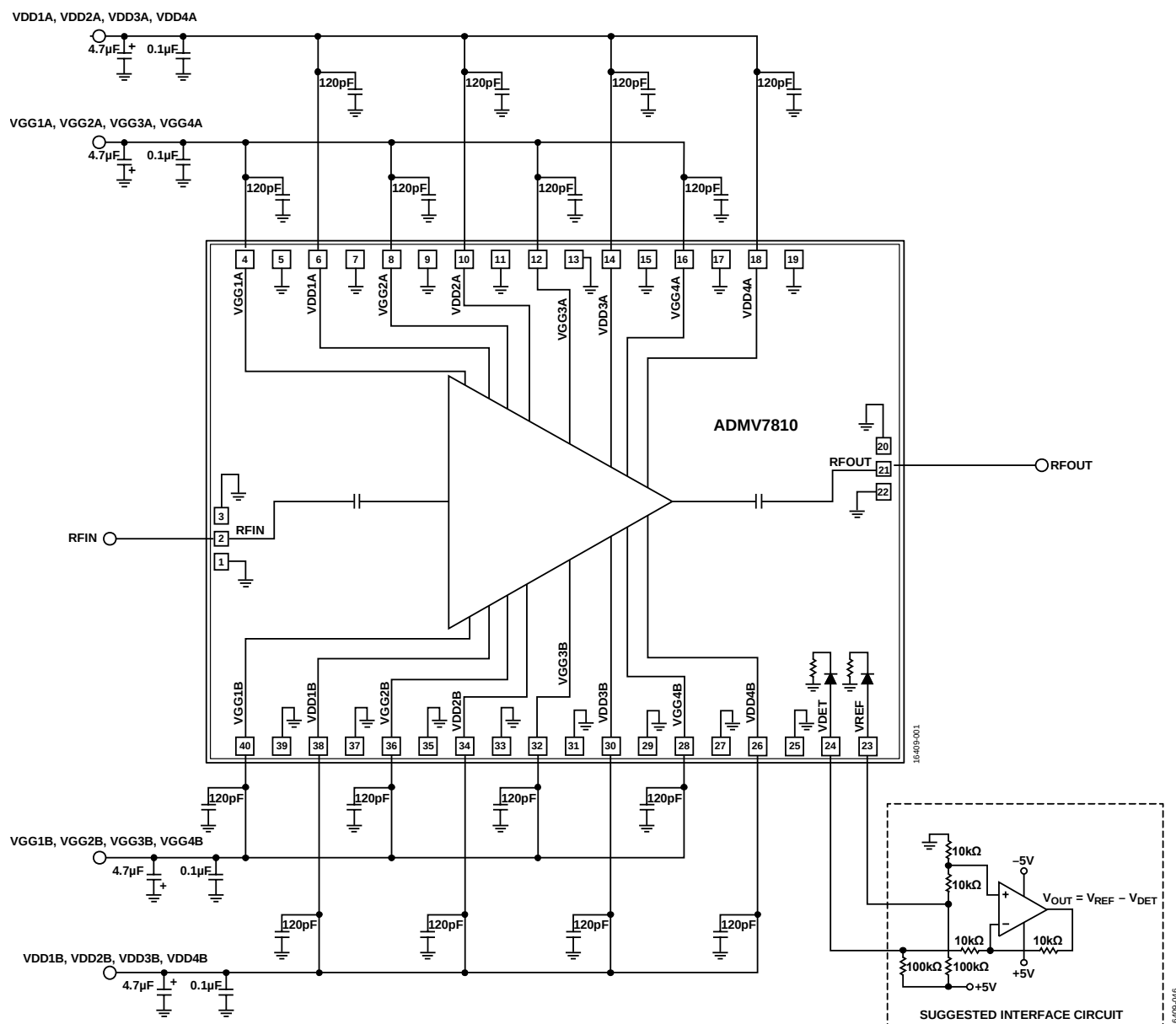
Figure 47. Typical Application Circuit
