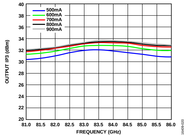
Figure 20. Output IP3 vs. Frequency over I_{DD} , P_{OUT}/\text{Tone} = 14 \text{ dBm}
