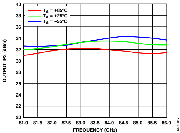
Figure 17. Output IP3 vs. Frequency over Various Temperatures, I_{DD} = 800 \text{ mA} , P_{OUT}/\text{Tone} = 14 \text{ dBm}
