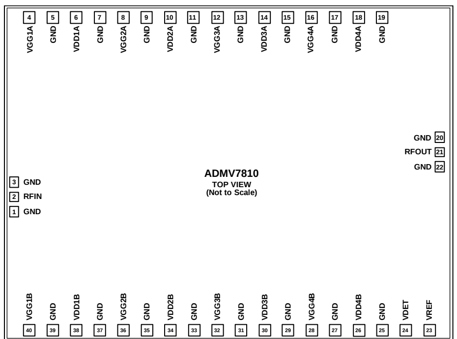
Figure 2. Pad Configuration
