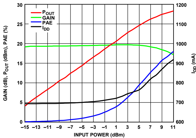
Figure 28. Gain, P_{OUT} , PAE, and I_{DD} vs. Input Power, RF = 81 GHz, I_{DD} = 700 mA
