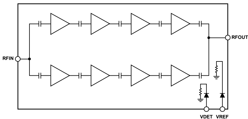
Figure 46. Power Amplifier Circuit Architecture
