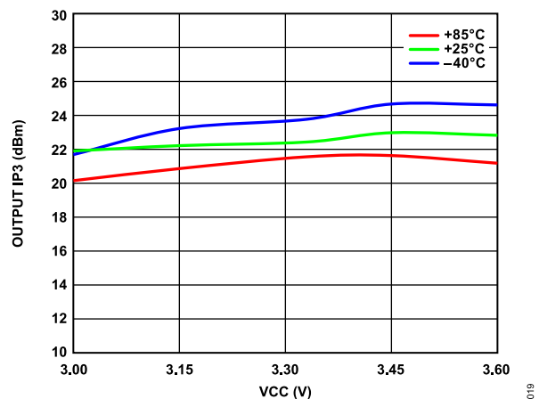
Figure 16. Output IP3 vs. VCC over Temperature
