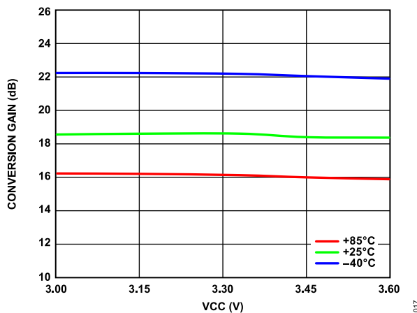
Figure 14. Conversion Gain vs. VCC over Temperature
