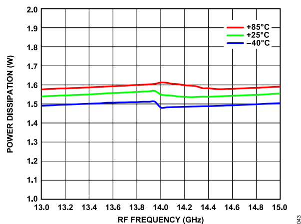
Figure 41. Power Dissipation vs. RF Frequency over Temperature
