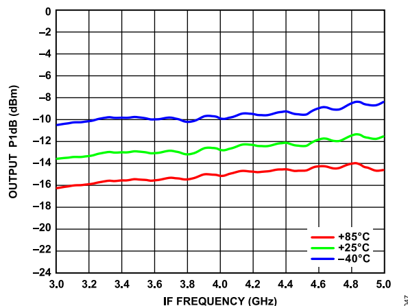
Figure 45. Output P1dB vs. IF Frequency over Temperature
