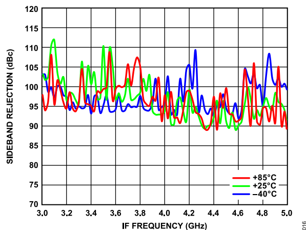
Figure 13. Sideband Rejection vs. IF Frequency over Temperature
