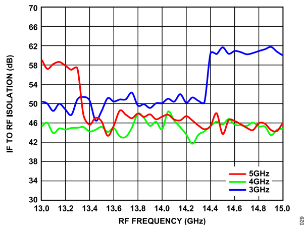
Figure 26. IF to RF Isolation vs. RF Frequency, IF = 3 GHz, 4 GHz, and 5 GHz
