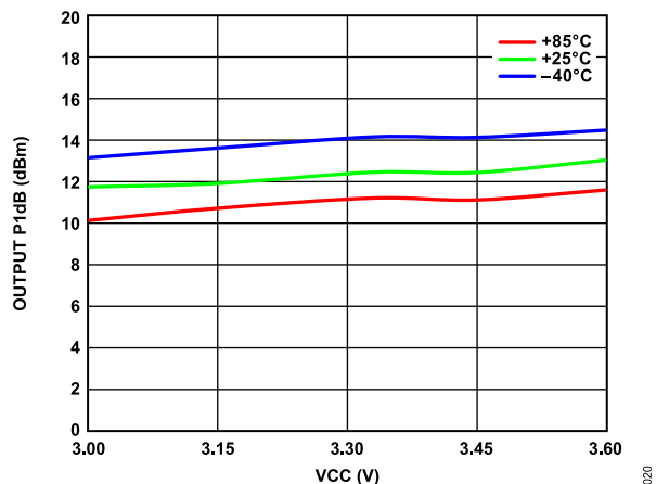
Figure 17. Output P1dB vs. VCC over Temperature
