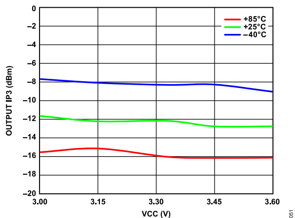
Figure 49. Output IP3 vs. VCC over Temperature
