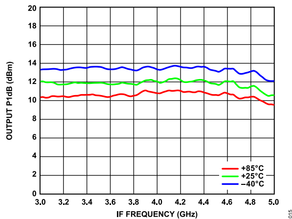
Figure 12. Output P1dB vs. IF Frequency over Temperature
