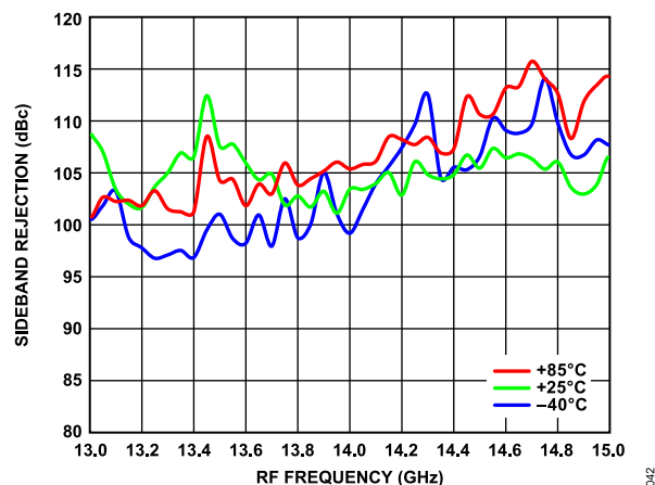
Figure 40. Sideband Rejection vs. RF Frequency over Temperature
