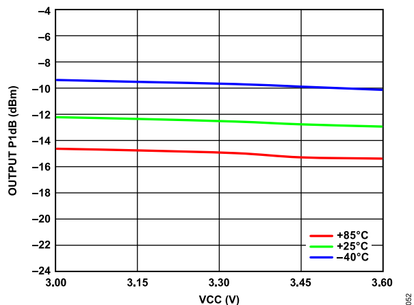
Figure 50. Output P1dB vs. VCC over Temperature
