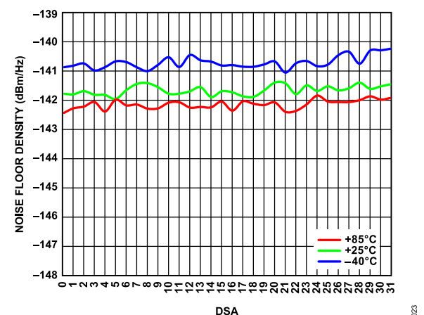
Figure 20. Noise Floor Density vs. DSA over Temperature
