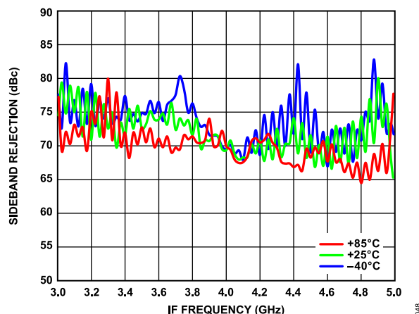
Figure 46. Sideband Rejection vs. IF Frequency over Temperature
