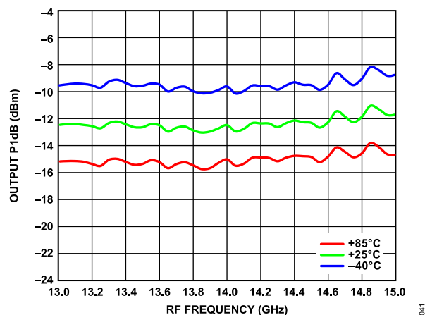
Figure 39. Output P1dB vs. RF Frequency over Temperature
