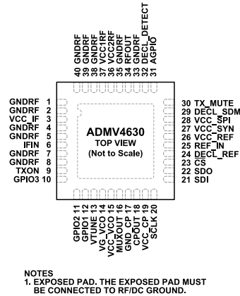
Figure 2. Pin Configuration
