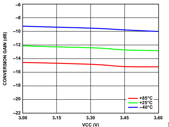
Figure 47. Conversion Gain vs. VCC Frequency over Temperature
