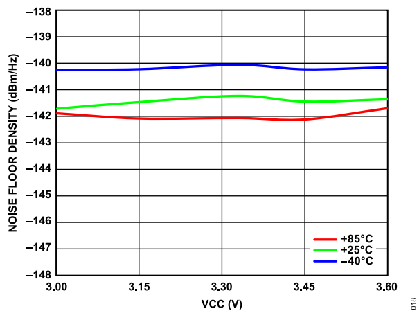
Figure 15. Noise Floor Density vs. VCC over Temperature
