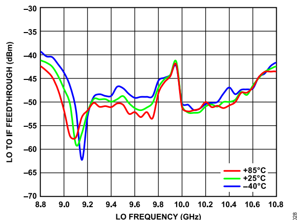
Figure 25. LO to IF Feedthrough vs. LO Frequency over Temperature
