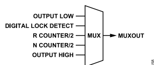
Figure 59. MUXOUT Pin Diagram
