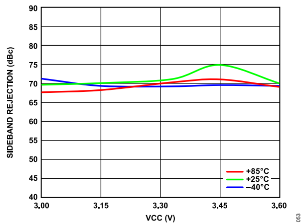
Figure 51. Sideband Rejection vs. VCC over Temperature
