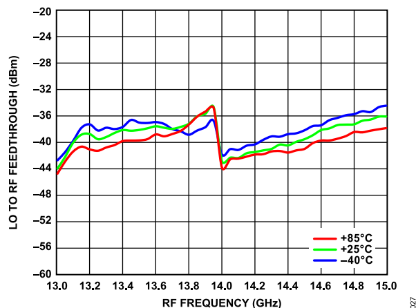
Figure 24. LO to RF Feedthrough vs. RF Frequency over Temperature
