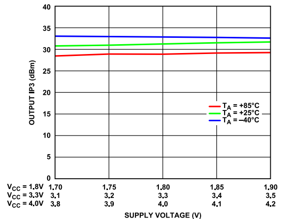
Figure 40. Output IP3 vs. Supply Voltage over Temperature
