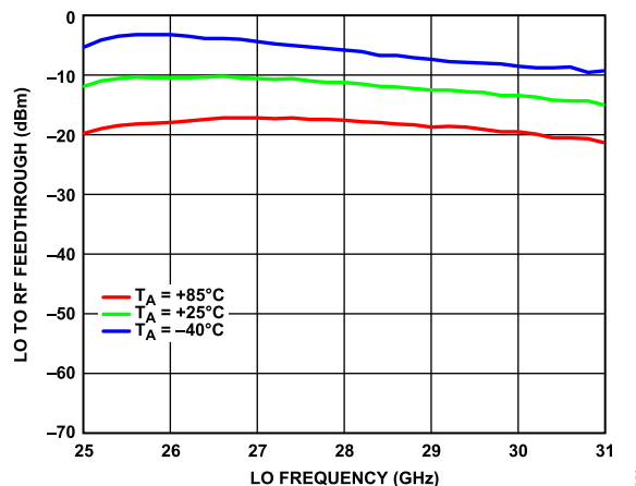
Figure 63. LO to RF Feedthrough vs. LO Frequency, Uncalibrated over Temperature
