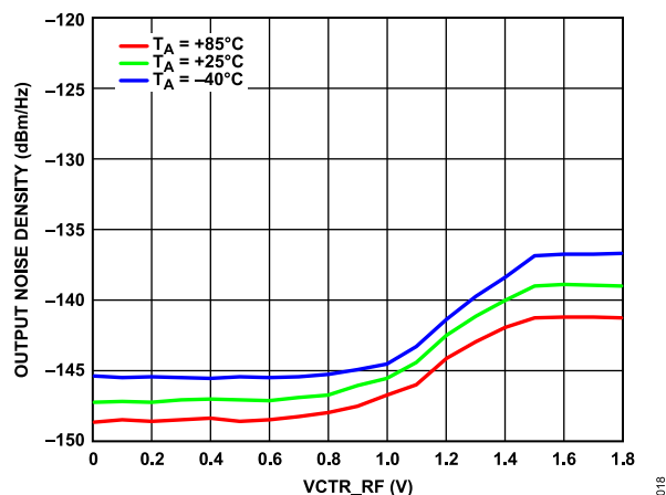
Figure 18. Output Noise Density vs. V_{CTR\_RF} over Temperature
