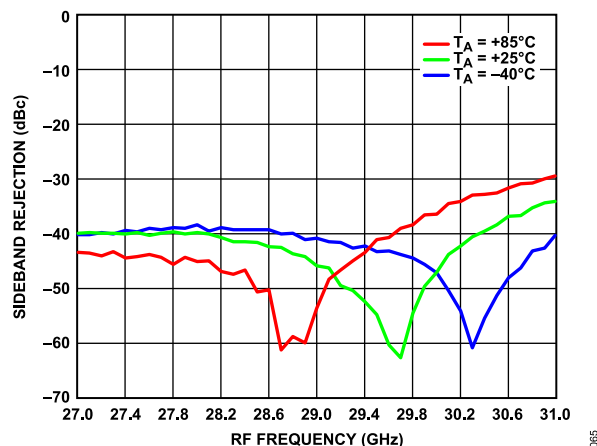
Figure 56. Sideband Rejection vs. RF Frequency over Temperature, Calibrated with RF Frequency = 30 GHz, IF Mode, VCTR_RF = 1.8 V, T_A = 25^\circ\text{C}
