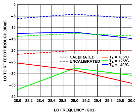
Figure 57. LO to RF Feedthrough vs. LO Frequency, Calibrated at T_A = 25^\circ\text{C} and Not Calibrated, over Temperature
