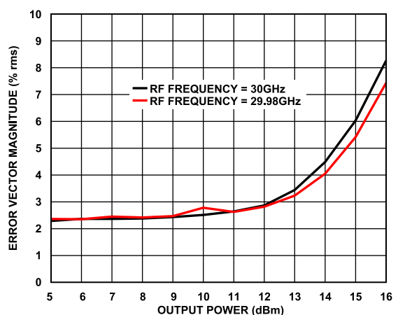
Figure 97. Error Vector Magnitude vs. Output Power, 8 QPSK Modulation, 12 MHz Bandwidth
