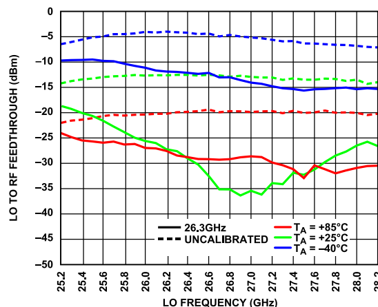
Figure 59. LO to RF Feedthrough vs. LO Frequency, over Temperature, Not Calibrated and Calibrated with LO Frequency = 26.3 GHz at T_A = 25^\circ\text{C} , IF Mode
