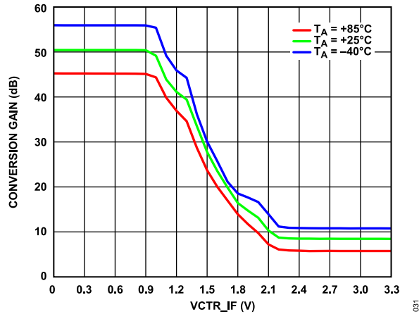
Figure 38. Conversion Gain vs. VCTR_IF over Temperature
