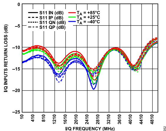
Figure 62. I/Q Inputs Return Loss vs. I/Q Frequency, Single-Ended over Temperature (S11 Is Return Loss)
