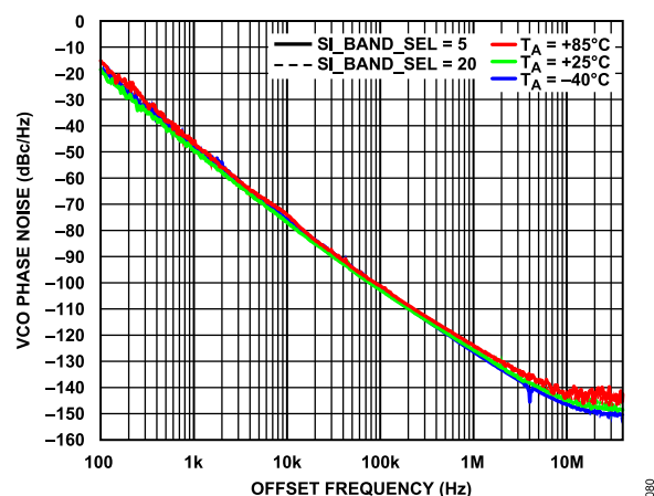
Figure 77. VCO Phase Noise vs. Offset Frequency over Temperature, Open Loop, VTUNE = 1.4 V, SI_BAND_SEL = 5 and 20
