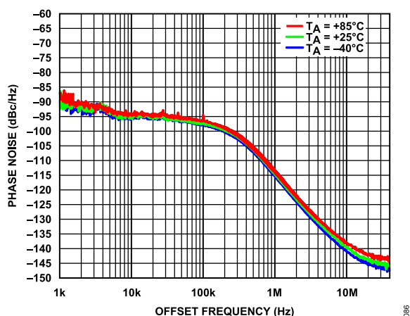
Figure 83. Phase Noise vs. Offset Frequency over Temperature, LO Frequency = 26.8 GHz, R\_WORD = 4 , CP\_CURRENT = 2.1 mA
