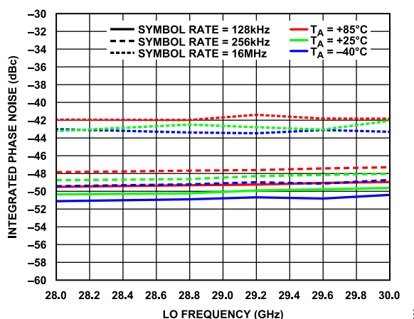
Figure 80. Integrated Phase Noise vs. LO Frequency over Temperature, R_WORD = 2, CP_CURRENT = 4.2 mA, Integrated from 1% to 50% of the Symbol Rate
