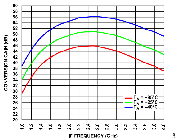
Figure 37. Conversion Gain vs. IF Frequency over Temperature
