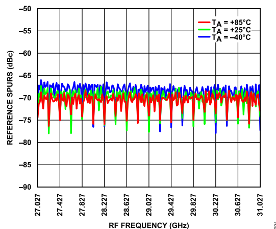
Figure 87. Reference Spurs vs. RF Frequency over Temperature, I/Q Mode, R\_WORD = 2 , CP\_CURRENT = 2.1 mA, P_{OUT} = 10 dBm
