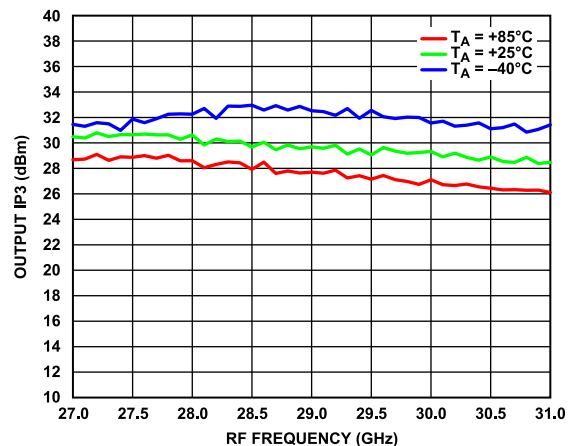
Figure 9. Output IP3 vs. RF Frequency over Temperature
