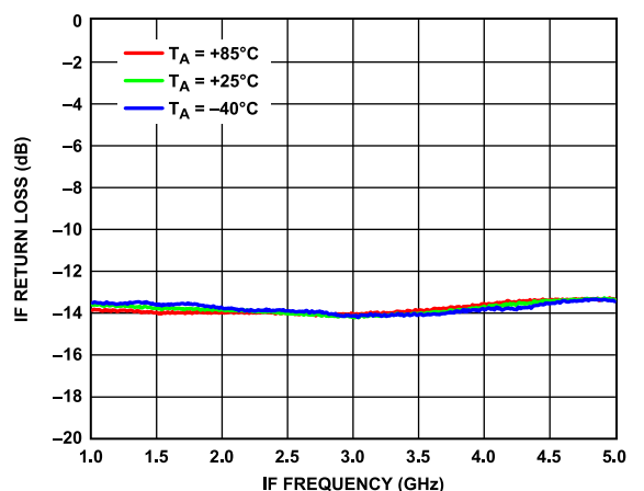
Figure 64. IF Input Return Loss vs. IF Frequency over Temperature
