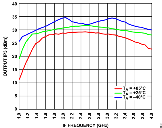
Figure 39. Output IP3 vs. IF Frequency over Temperature
