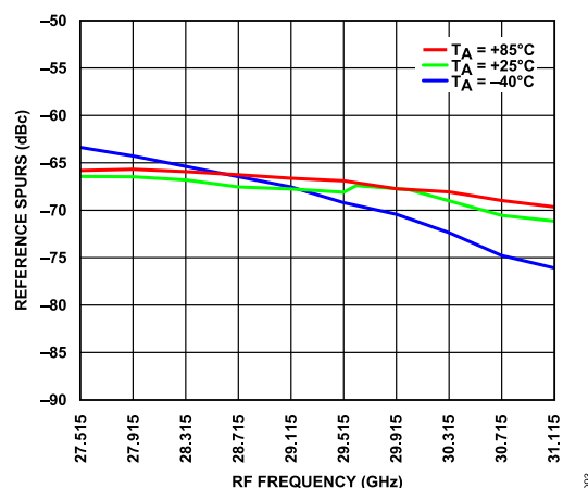
Figure 86. Reference Spurs vs. RF Frequency over Temperature, IF Mode, R\_WORD = 4 , CP\_CURRENT = 2.1 mA, VCTR\_IF = 0 V, P_{OUT} = 10 dBm
