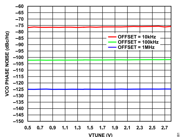
Figure 78. VCO Phase Noise vs. VTUNE for Various Offsets, Open Loop, TA = 25°C
