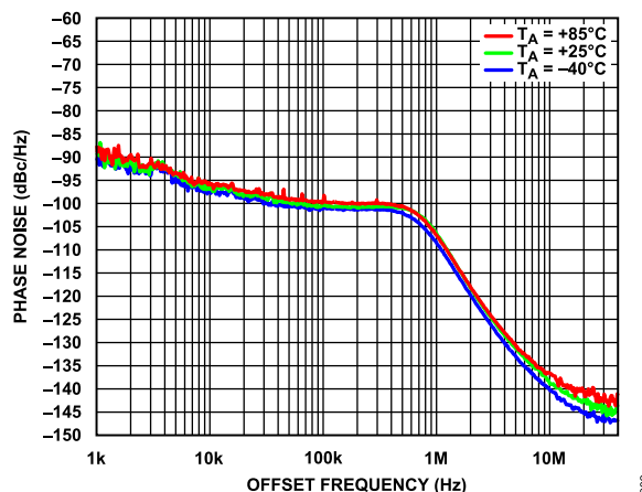
Figure 79. Phase Noise vs. Offset Frequency over Temperature, R_WORD = 2, CP_CURRENT = 4.2 mA, LO Frequency = 30 GHz
