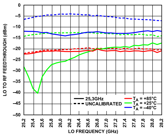
Figure 58. LO to RF Feedthrough vs. LO Frequency, over Temperature, Not Calibrated and Calibrated with LO Frequency = 25.3 GHz at T_A = 25^\circ\text{C} , IF Mode
