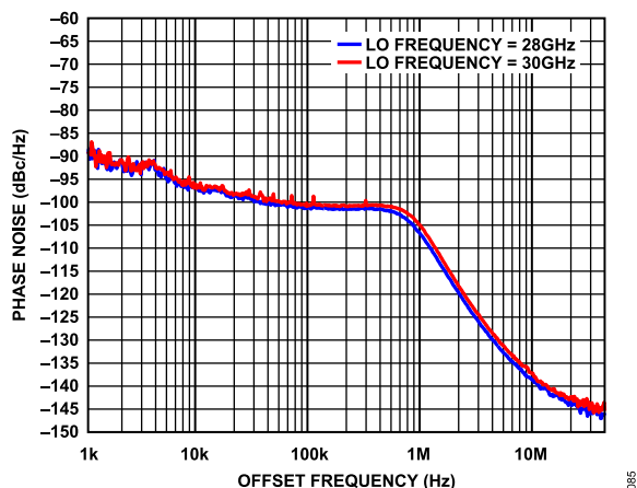
Figure 82. Phase Noise vs. Offset Frequency, R\_WORD = 2 , CP\_CURRENT = 4.2 mA, LO Frequency = 28 GHz and 30 GHz
