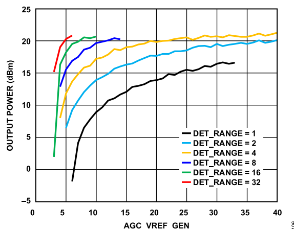
Figure 96. AGC Voltage Reference Sweep
