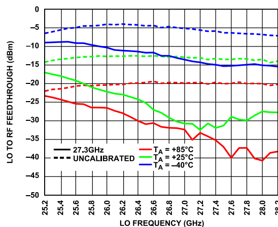
Figure 60. LO to RF Feedthrough vs. LO Frequency, over Temperature, Not Calibrated and Calibrated with LO Frequency = 27.3 GHz at T_A = 25^\circ\text{C} , IF Mode
