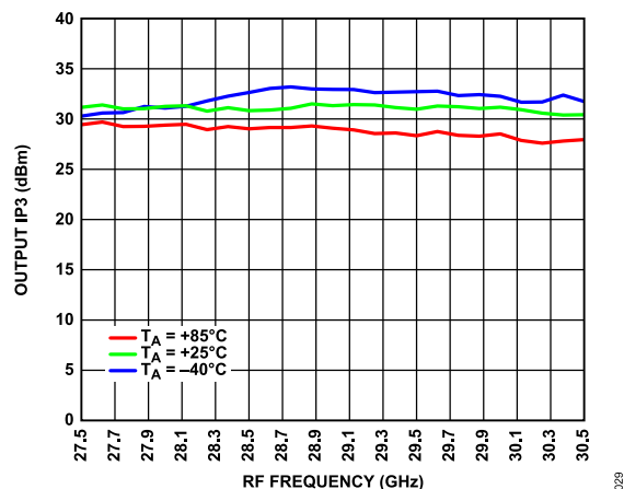
Figure 36. Output IP3 vs. RF Frequency over Temperature
