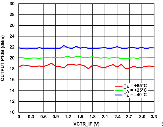
Figure 54. Output P1dB vs. VCTR_IF over Temperature
