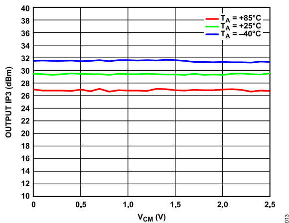
Figure 13. Output IP3 vs. V_{CM} over Temperature
