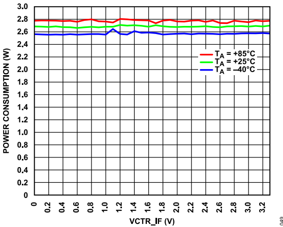
Figure 55. Power Consumption vs. VCTR_IF over Temperature at Compression POUT
