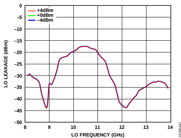
Figure 40. LO Leakage at IF Output vs. LO Frequency at Various LO Powers
