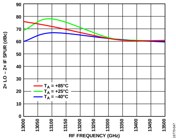
Figure 47. 2x LO - 2x IF Leakage vs. RF Frequency at Various Temperatures, IF = 3.1 GHz, -10 dBm
