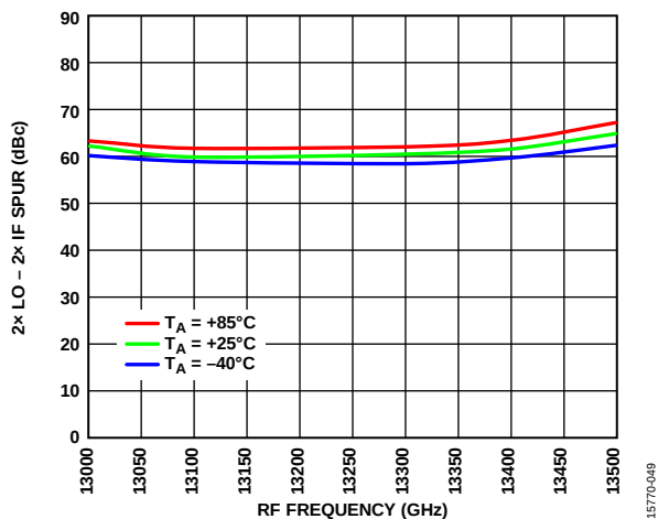
Figure 49. 2x LO - 2x IF Leakage vs. RF Frequency at Various Temperatures, IF = 3.5 GHz, -10 dBm
