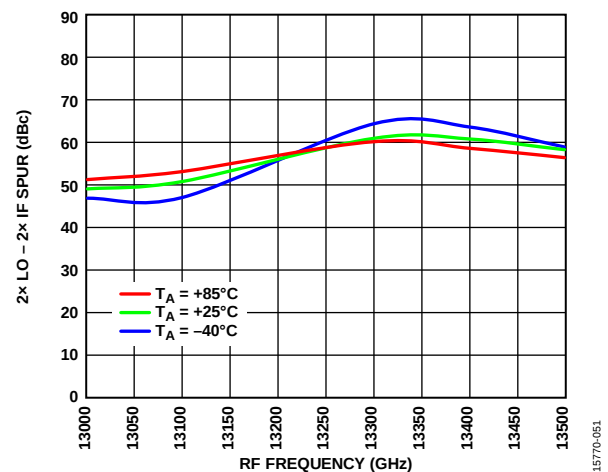
Figure 51. 2x LO - 2x IF Leakage vs. RF Frequency at Various Temperatures, IF = 3.3 GHz, 0 dBm
