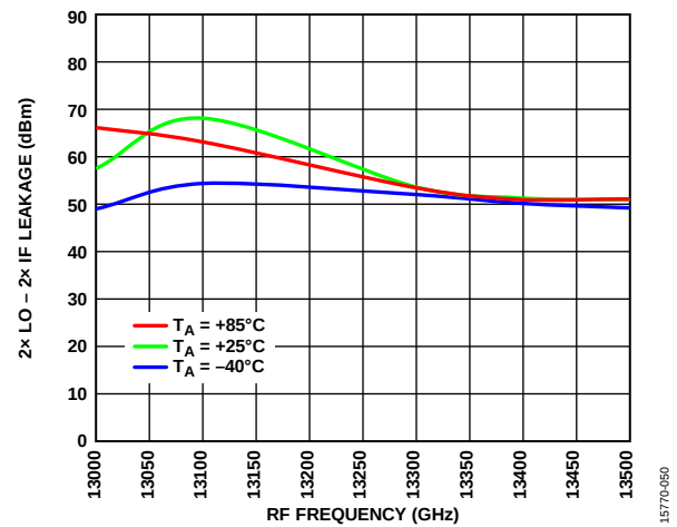
Figure 50. 2x LO - 2x IF Leakage vs. RF Frequency at Various Temperatures, IF = 3.1 GHz, 0 dBm
