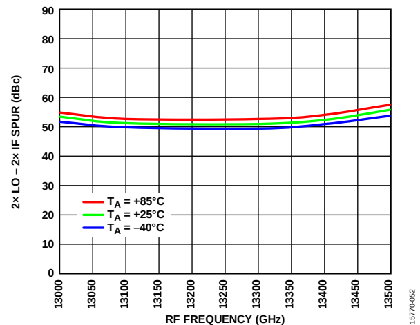
Figure 52. 2x LO - 2x IF Leakage vs. RF Frequency at Various Temperatures, IF = 3.5 GHz, 0 dBm
