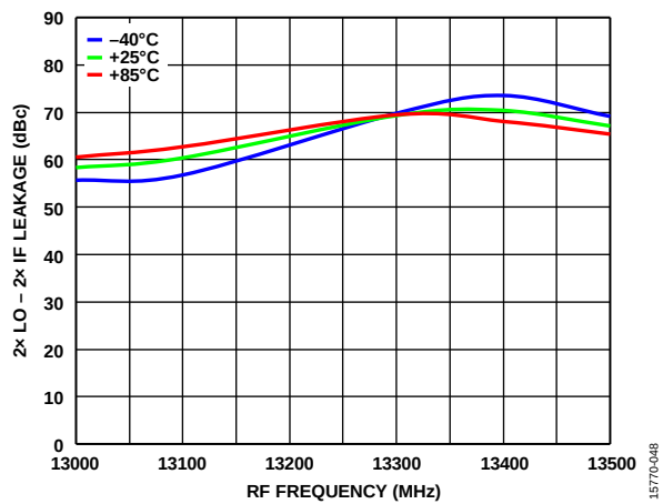
Figure 48. 2x LO - 2x IF Leakage vs. RF Frequency at Various Temperatures, IF = 3.3 GHz, -10 dBm
