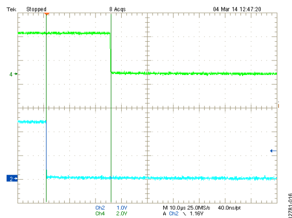
Figure 16. OUT Propagation Delay With VCC/VIN Falling
