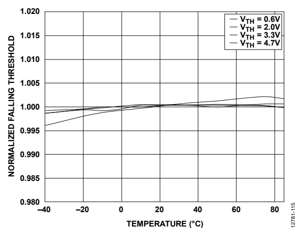
Figure 9. Normalized Falling Threshold vs. Temperature
