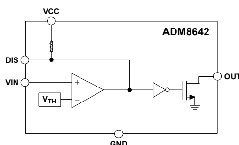
Figure 2. ADM8642 Functional Block Diagram
