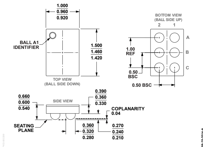
Figure 37. 6-Ball Wafer Level Chip Scale Package [WLCSP] (CB-6-17)
