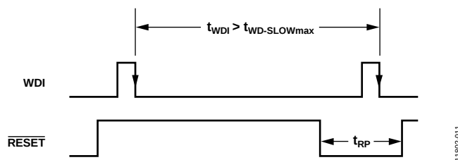
Figure 22. Watchdog Slow Timeout Fault
