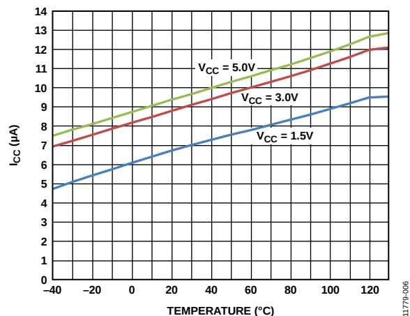
Figure 6. Supply Current ( I_{CC} ) vs. Temperature
