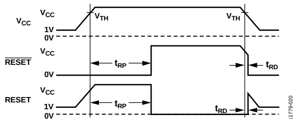
Figure 20. Reset Timing Diagram
