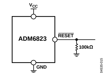
Figure 13. Ensuring Reset Valid to V_{CC} = 0 V
