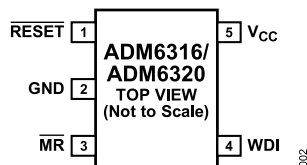
Figure 3. ADM6316/ADM6320 Pin Configuration
