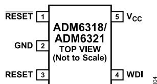
Figure 4. ADM6318/ADM6321 Pin Configuration
