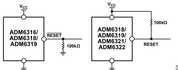
Figure 18. Ensuring Reset Valid to V_{CC} = 0 V
