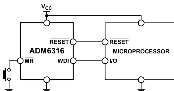
Figure 20. Typical Application Circuit
