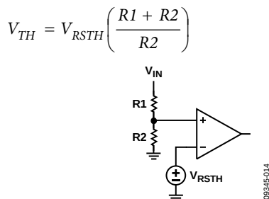
Figure 14. Setting the Adjustable Monitor
