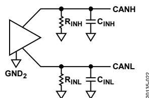
Figure 21. Input Resistance ( R_{INx} ) and Input Capacitance ( C_{INx} ) Measured in Recessive State, Bus Disconnected
