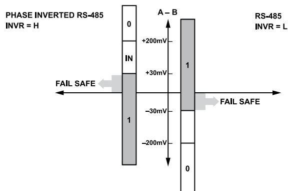
Figure 52. RS-485 and Phase Inverted RS-485 Comparison
