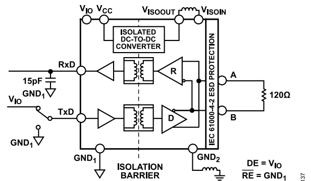
Figure 47. CMTI Test Diagram, Half Duplex
