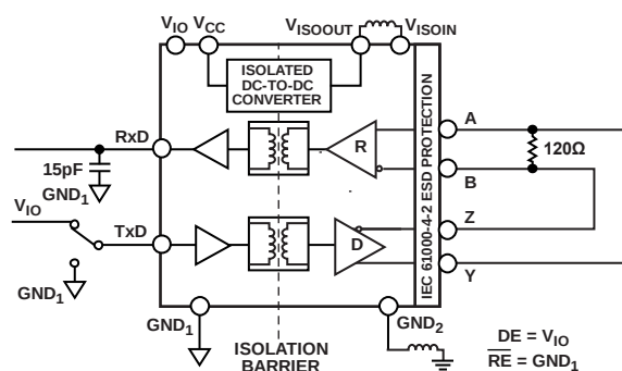
Figure 46. CMTI Test Diagram, Full Duplex
