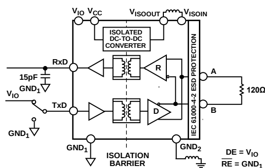
Figure 47. CMTI Test Diagram, Half Duplex
