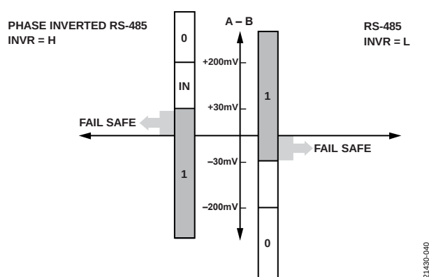
Figure 37. Noninverted RS-485 and Phase Inverted RS-485 Comparison
