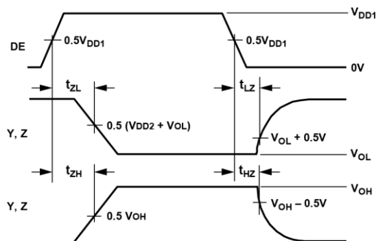
Figure 29. Receiver Propagation Delay
