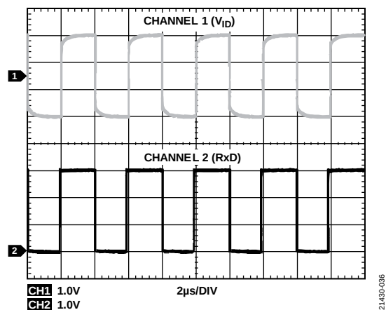
Figure 21. Receiver Switching at 500 kbps
