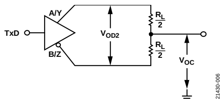
Figure 22. Driver Voltage Measurement |V_{OD2}|
