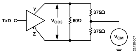
Figure 23. Driver Voltage Measurement over Common-Mode Range |V_{OD3}|
