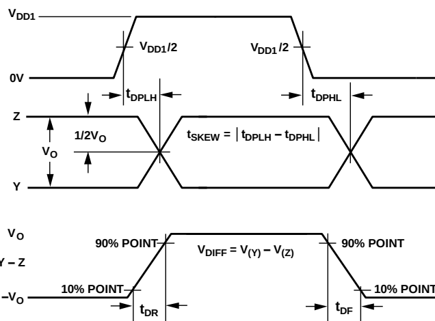
Figure 28. Driver Propagation Delay, Rise and Fall Timing
