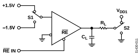
Figure 27. Receiver Enable or Disable Time Measurement
