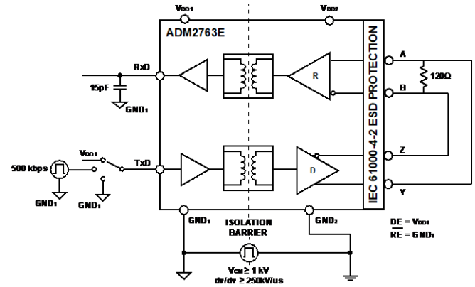
Figure 33. CMTI Test Diagram
