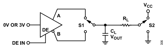
Figure 19. Driver Enable/Disable
