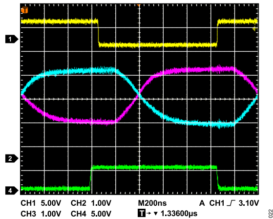
Figure 11. Driver/Receiver Propagation Delay, High to Low
