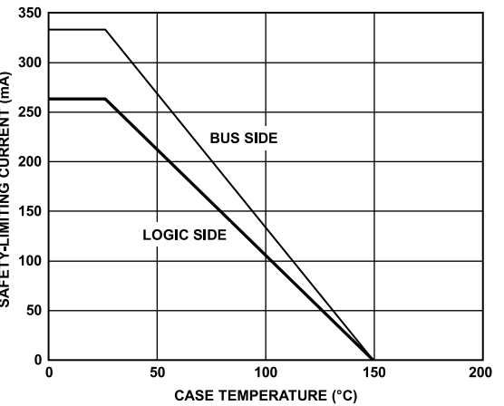
Figure 13. Thermal Derating Curve, Dependence of Safety-Limiting Values with Case Temperature per VDE 0884
