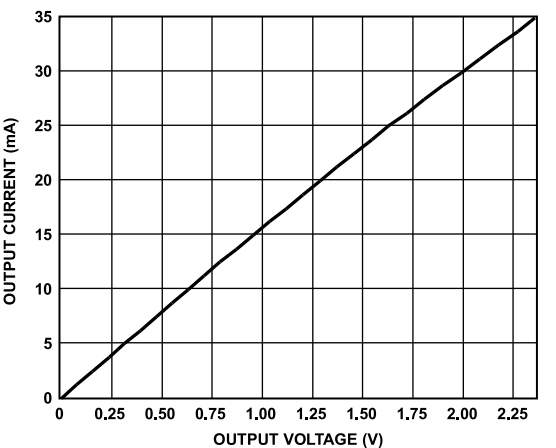
Figure 14. Output Current vs. Receiver Output Low Voltage
