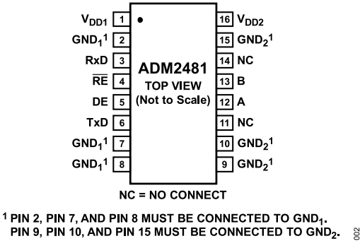
Figure 2. Pin Configuration
