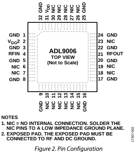
Figure 2. Pin Configuration
