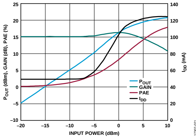
Figure 21. P_{OUT} , Gain, PAE, and I_{DD} vs. Input Power, 2 GHz, V_{DD} = 5\text{ V}
