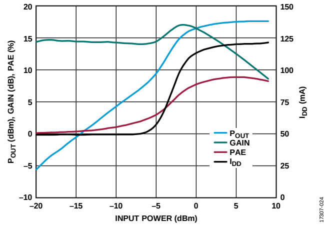
Figure 24. P_{OUT} , Gain, PAE, and I_{DD} vs. Input Power, 20 GHz, V_{DD} = 5\text{ V}
