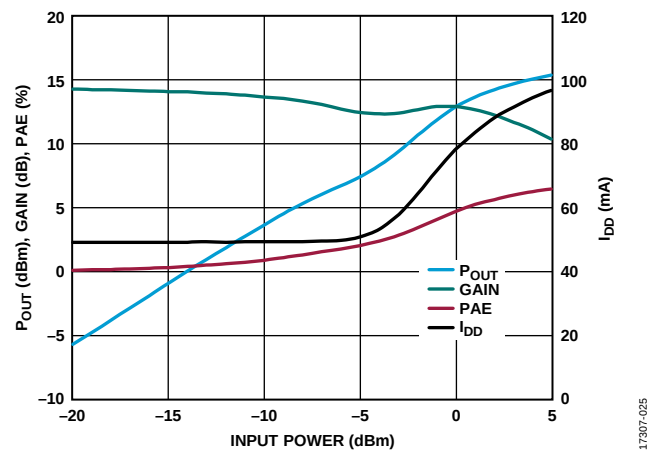
Figure 25. P_{OUT} , Gain, PAE, and I_{DD} vs. Input Power, 26 GHz, V_{DD} = 5\text{ V}
