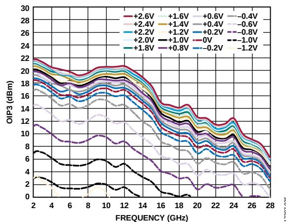
Figure 35. OIP3 vs. Frequency at Various V_{GG2} Voltages
