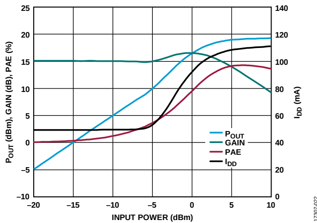
Figure 22. P_{OUT} , Gain, PAE, and I_{DD} vs. Input Power, 10 GHz, V_{DD} = 5\text{ V}
