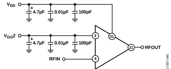
Figure 38. Typical Application Circuit
