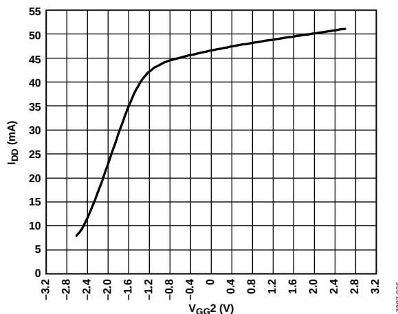
Figure 36. I_{DD} vs. V_{GG2} Voltages, V_{DD} = 5\text{ V}
