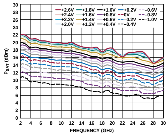
Figure 32. P_{SAT} vs. Frequency at Various V_{GG2} Voltages
