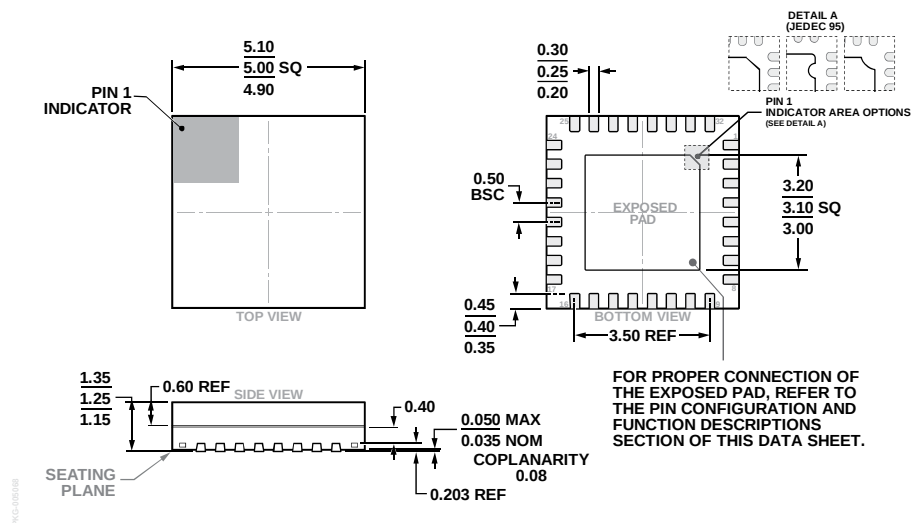
Figure 39. 32-Lead Lead Frame Chip Scale Package, Premolded Cavity [LFCSP_CAV] 5 mm × 5 mm Body and 1.25 mm Package Height (CG-32-2)
