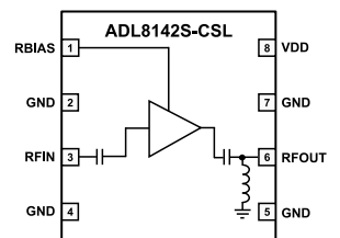
Figure 1. Functional Block Diagram
